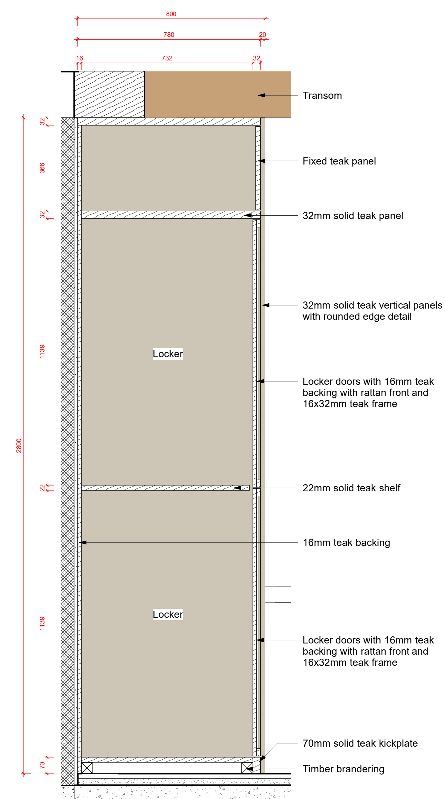
Section - Lockers | 1:10
