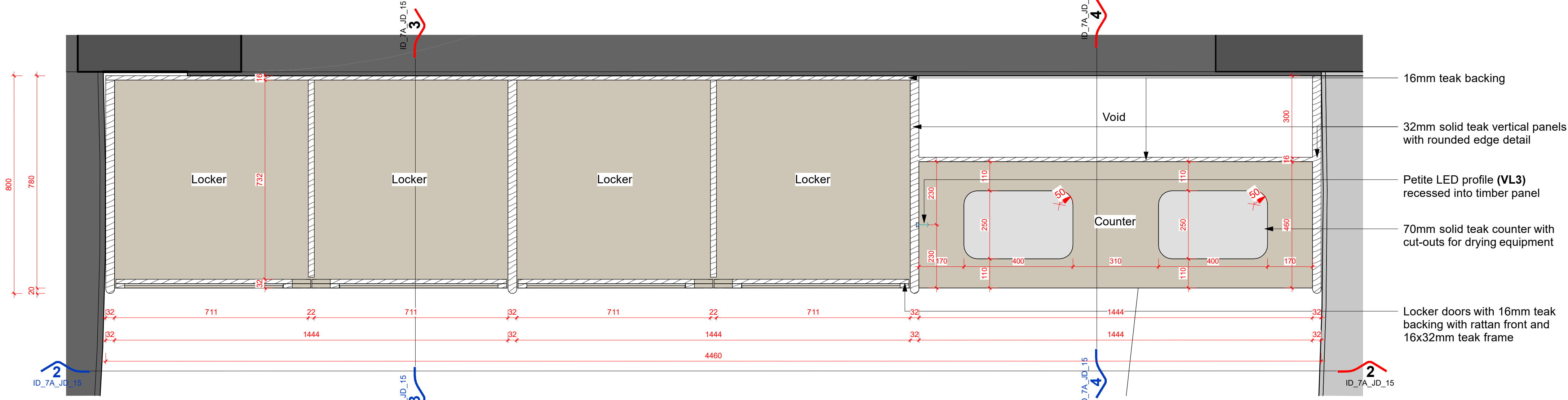
Floor Plan Lower Level - Lockers & Shelf | 1:10
