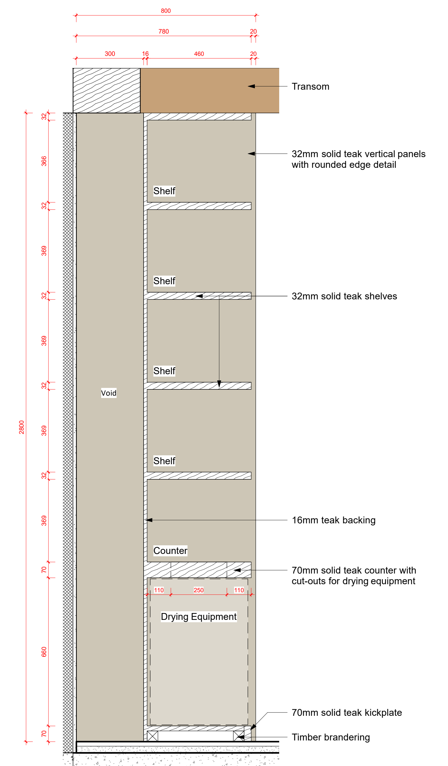
Section - Shelves | 1:10
