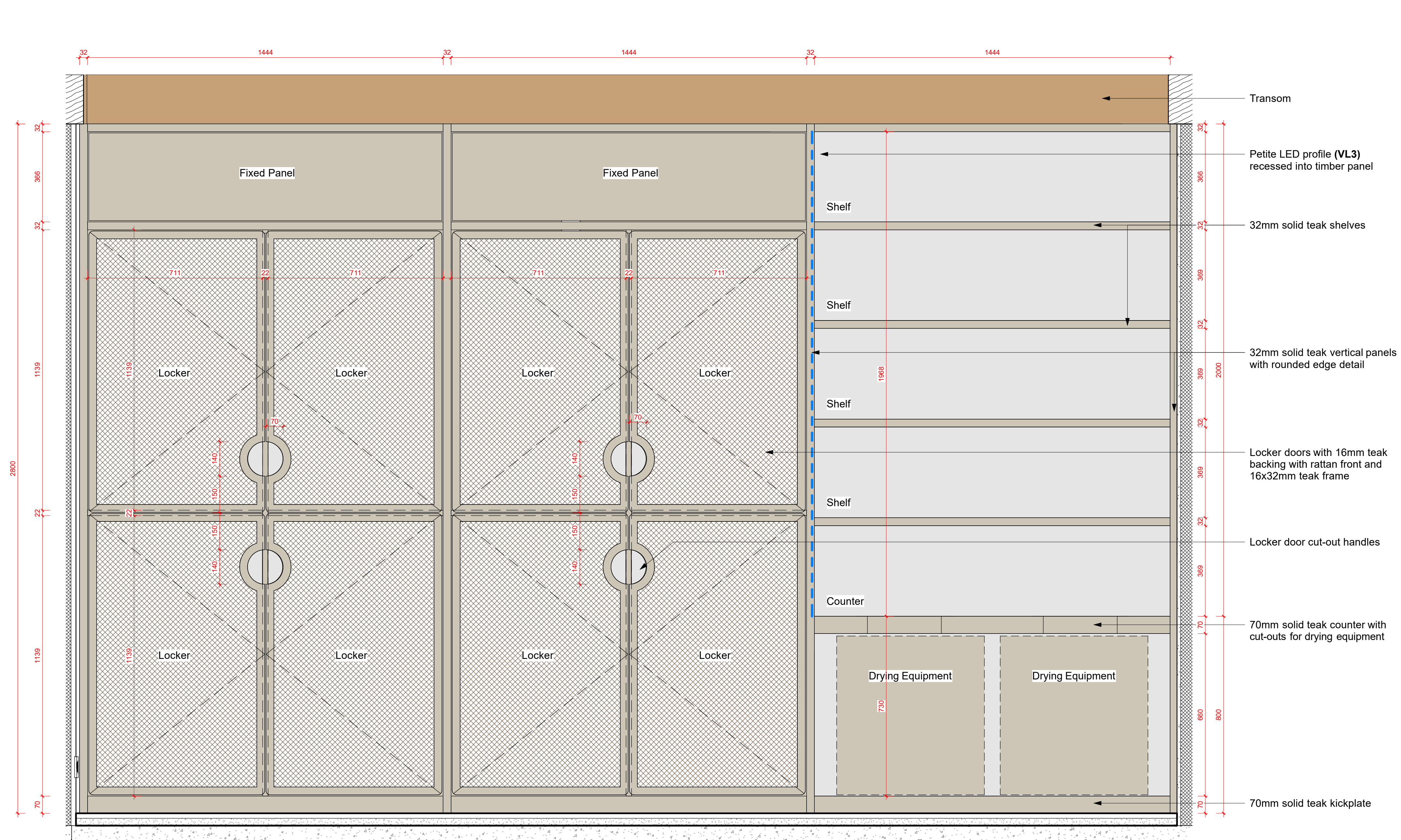
Front Elevation - Lockers & Shelf | 1:10
