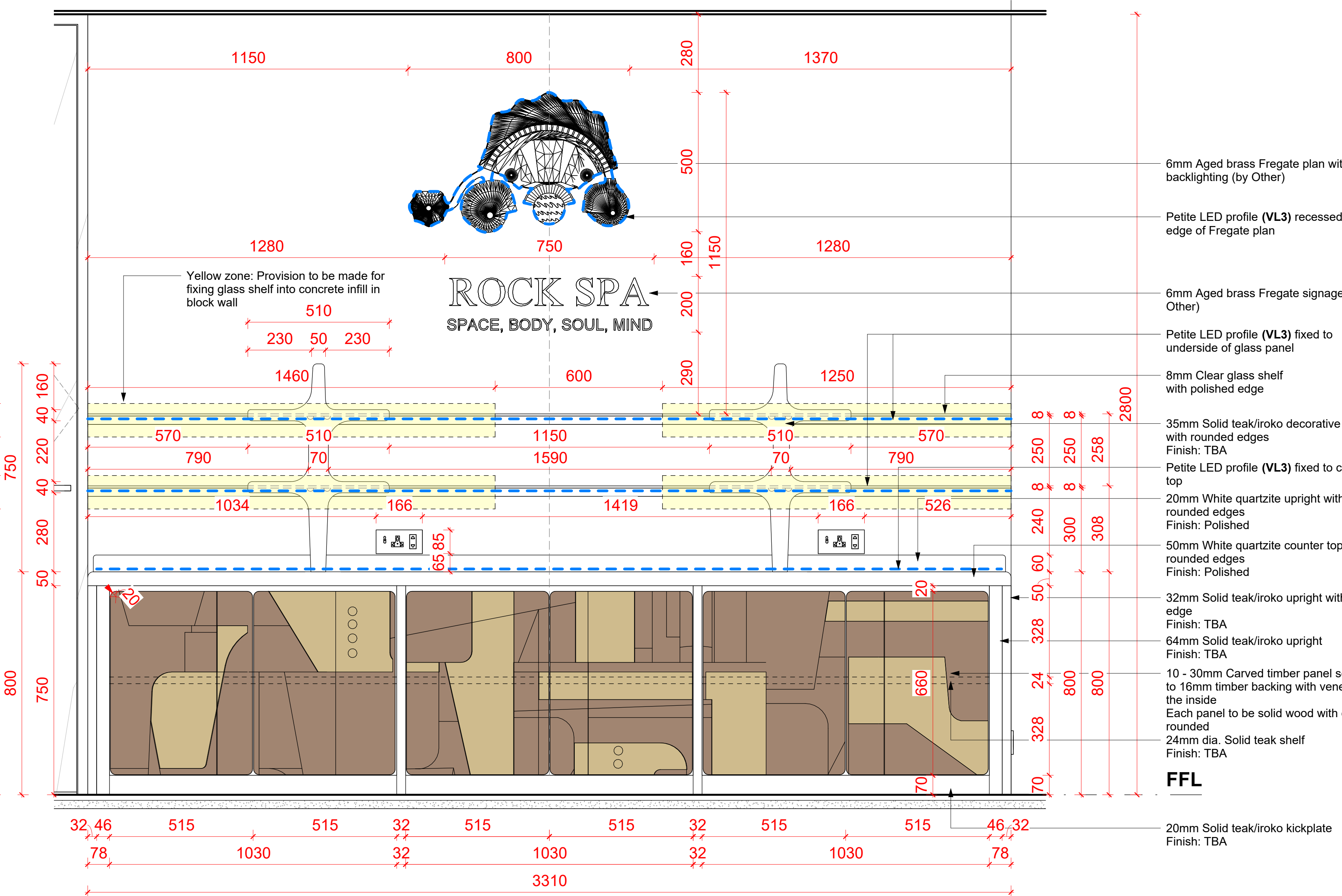
Front Elevation - Shelf B | 1:10
