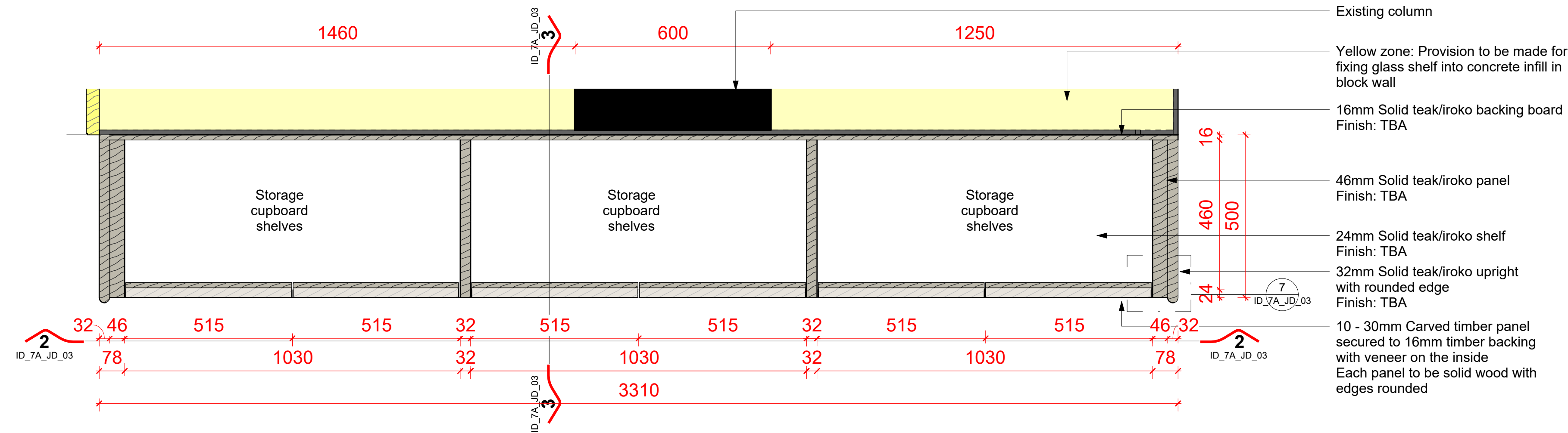
Floor Plan Lower Level - Cupboard | 1:10
