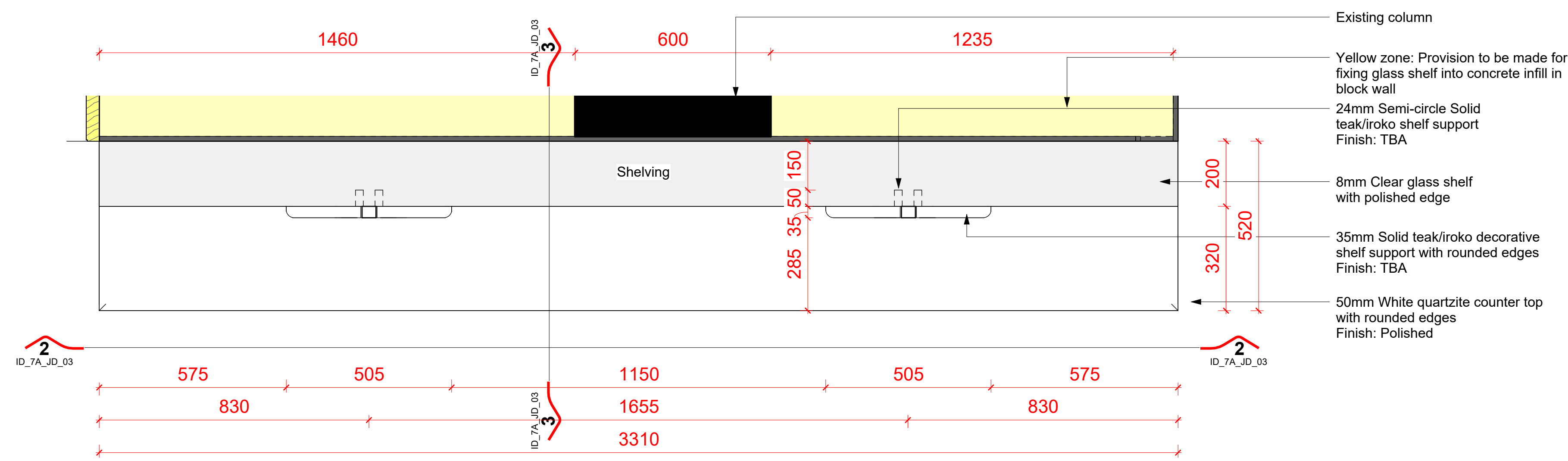
Floor Plan Upper Level - Glass Shelf | 1:10
