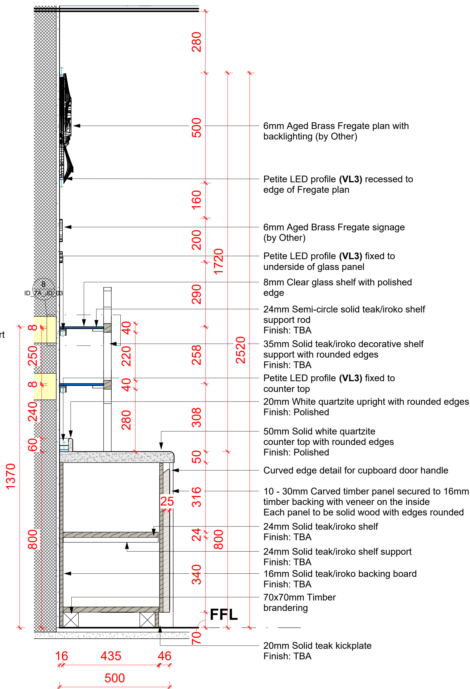
Section - Shelf B | 1:10
