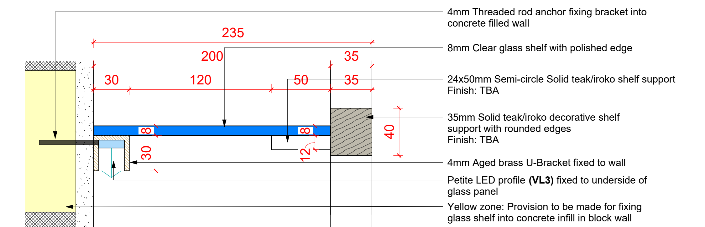
Section Callout - Glass shelf | 1:2
