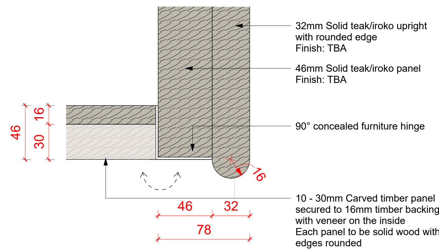
Plan Callout - Cupboard door corner | 1:2
