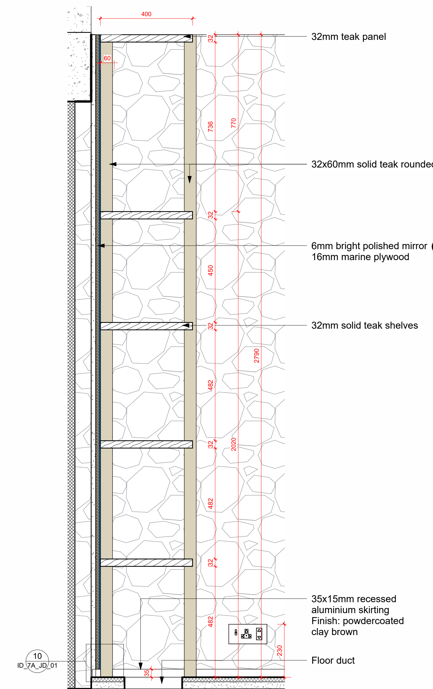
Section - Locker Shelves | 1:10
