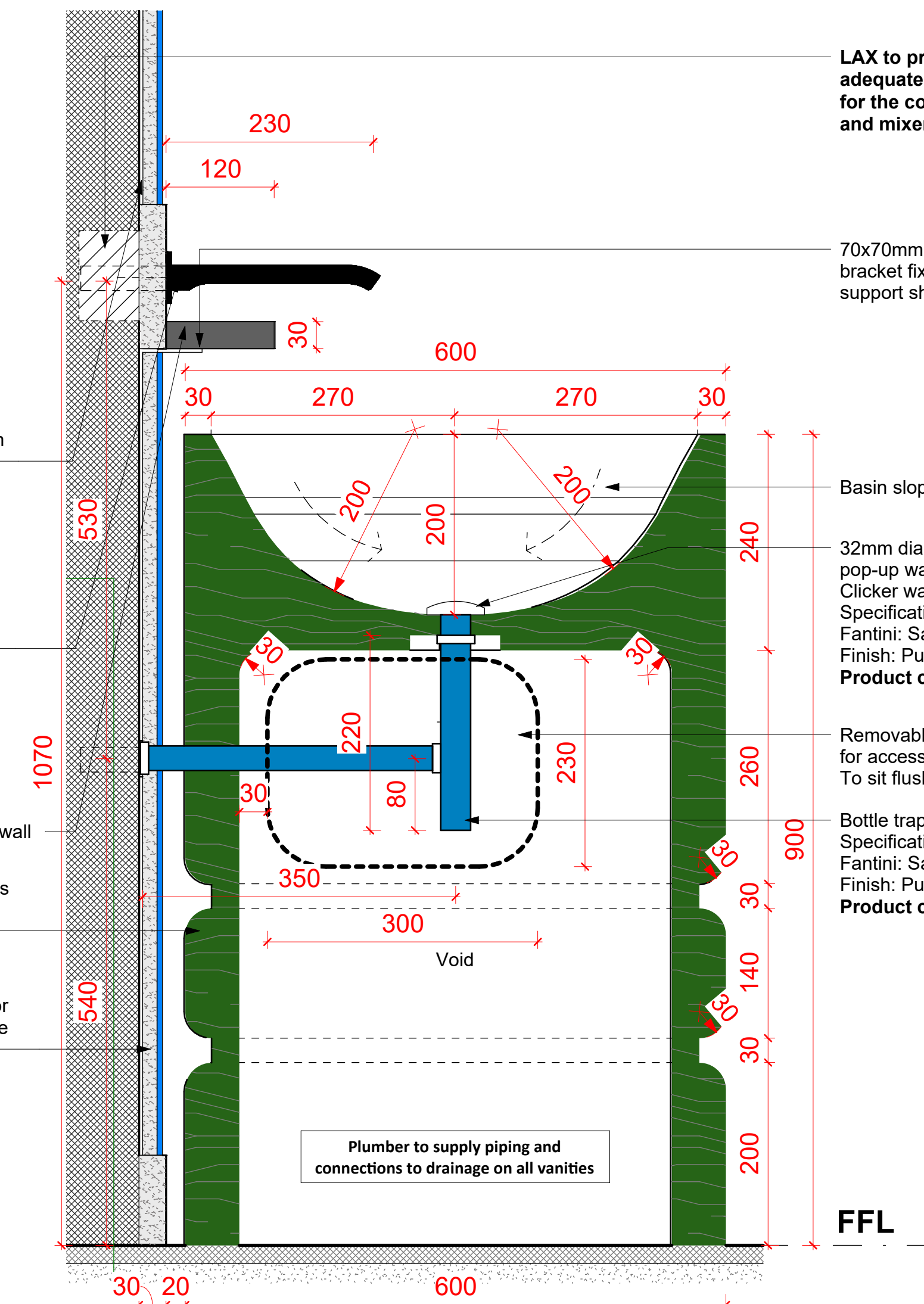
Section - Vanity | 1:5
