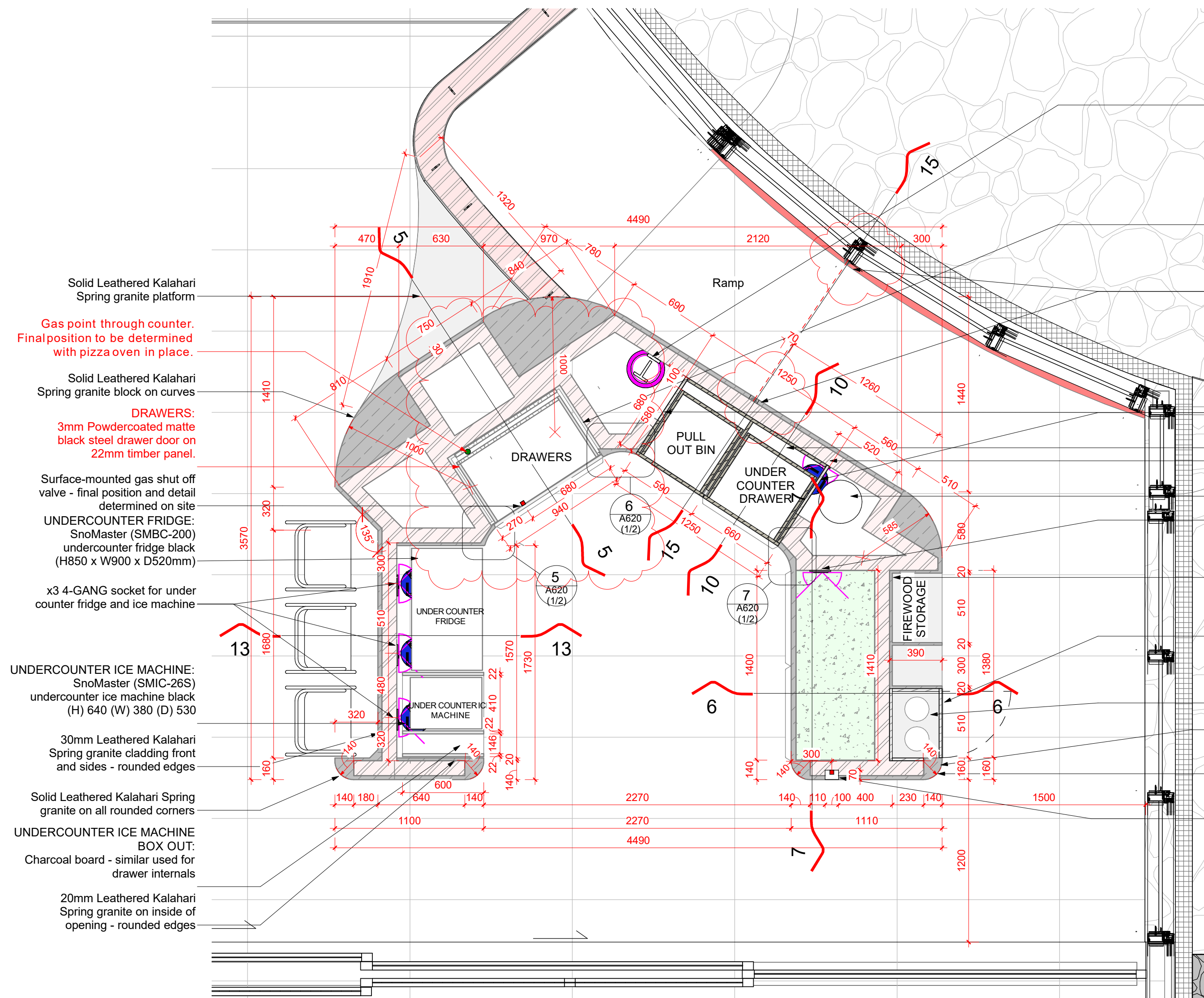
③ Plan Lower Level - Pavilion Cooking Station 1:25
