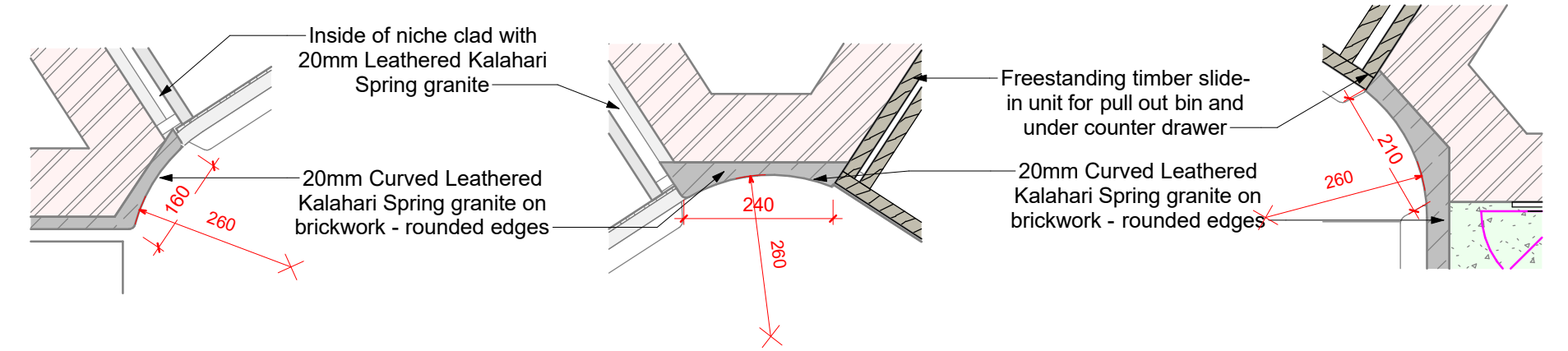
⑤ Plan Callout 01 - Granite Curve 1:10
