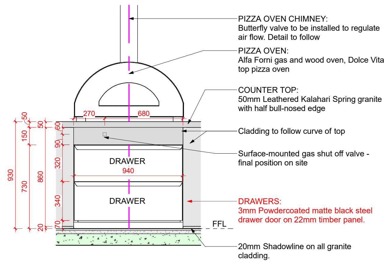
② Elevation 02 - Pizza Oven 1 : 20
