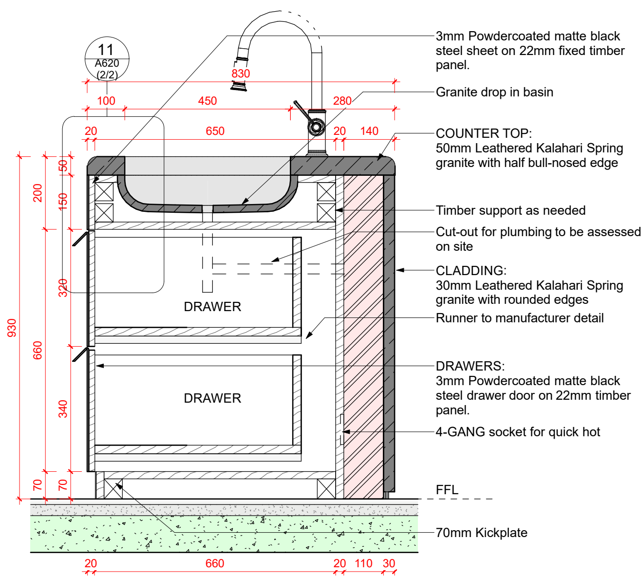
⑩ Section 04 - Drawers 1 : 10
