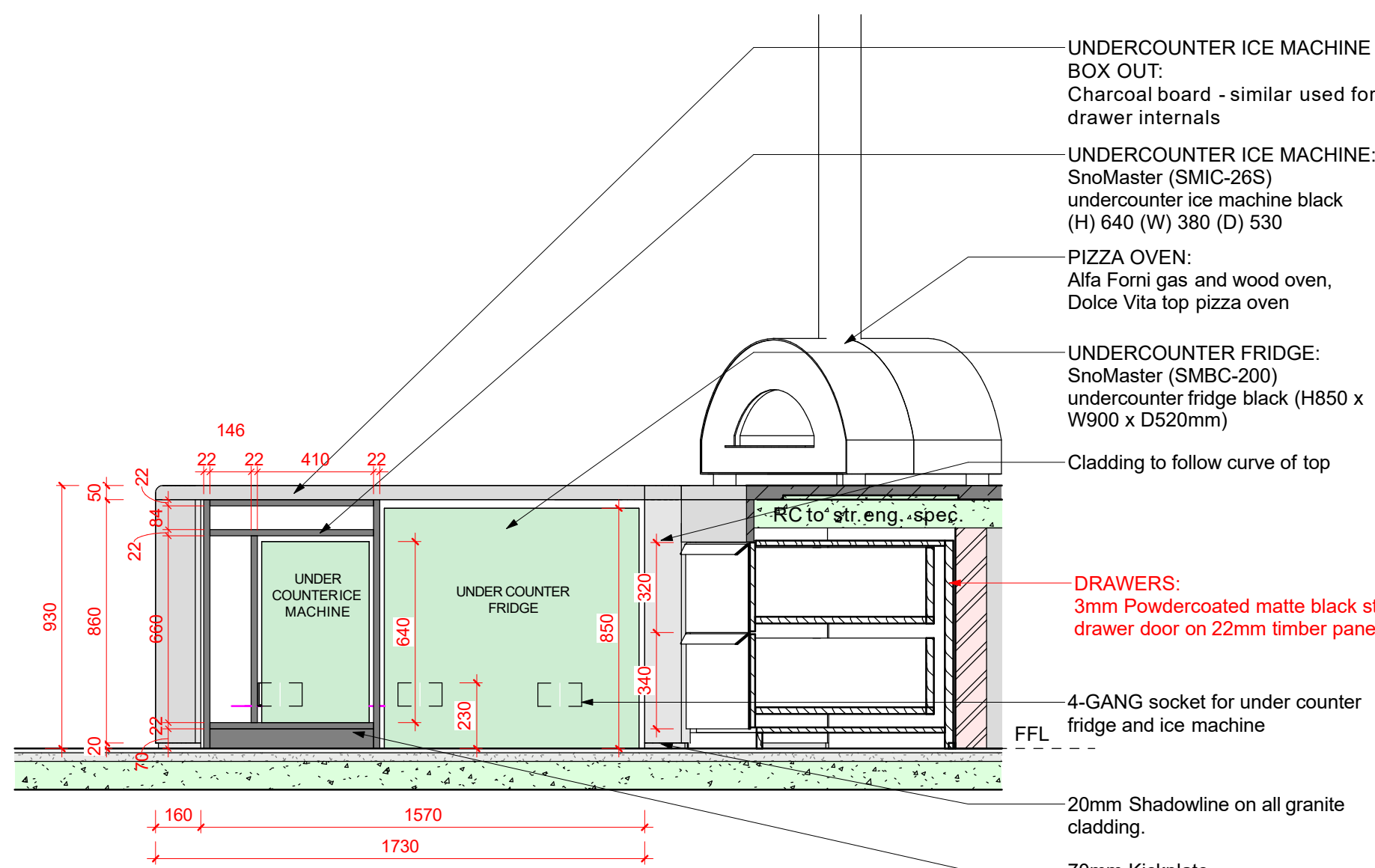
① Elevation 01 - Fridge & Freezer 1 : 20
