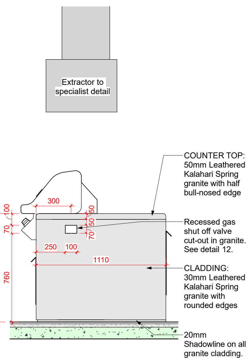
⑭ Elevation 06 - Gas Shut off valve 1 : 20
