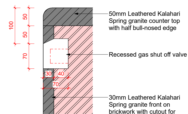
⑫ Callout - Recessed gas shut off valve 1 : 5
