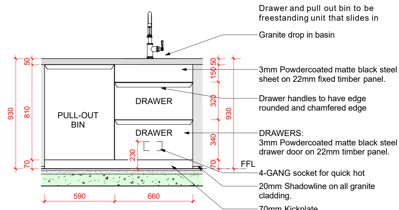
③ Elevation 03 - Drawers, Bin & Basin 1 : 20
