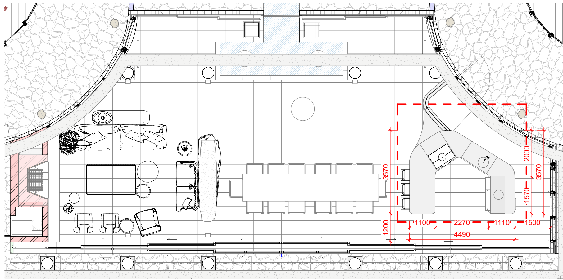
① Reference Plan - Pavilion - Cooking Station 1:100
