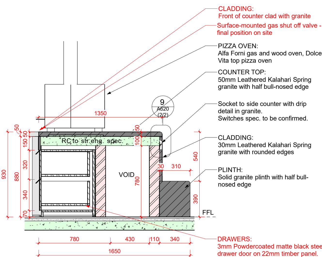
⑤ Section 01 - Pizza Oven & Pull-out Trolley 1 : 20
