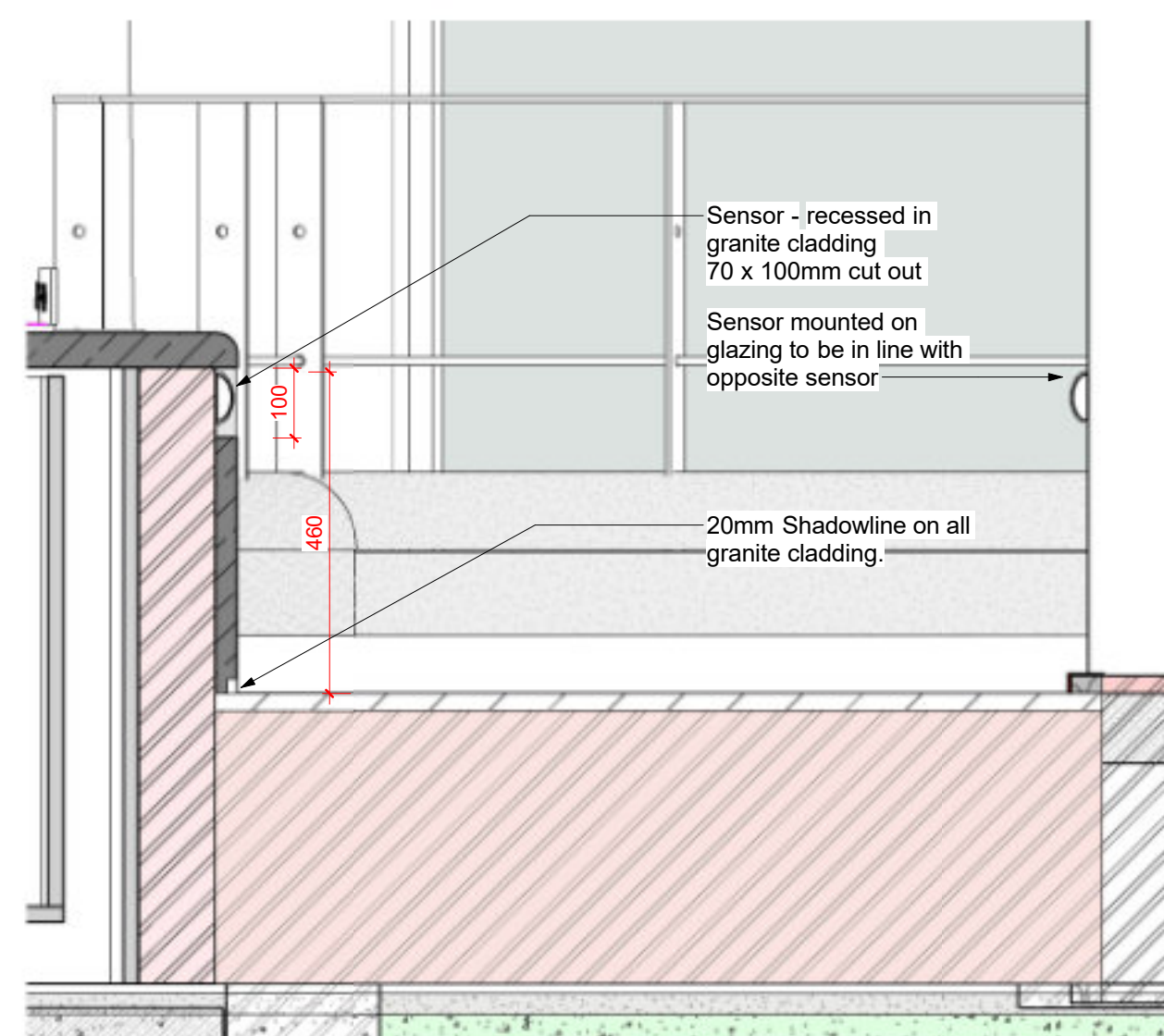
⑮ Section 05 - Sensor Position 1 : 10
