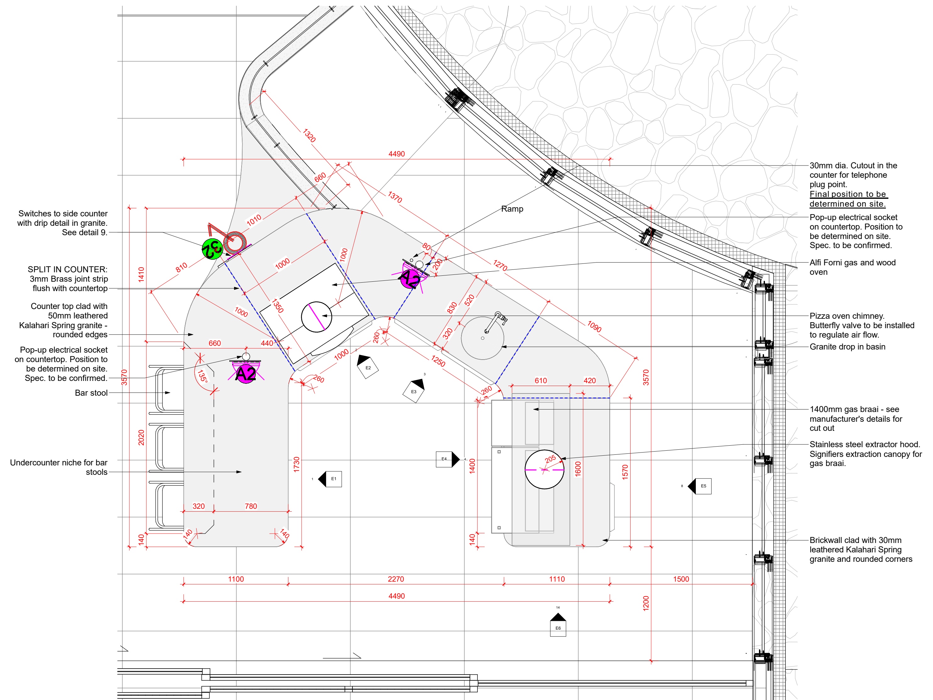
④ Plan Upper Level - Pavilion Cooking Station 1:25
