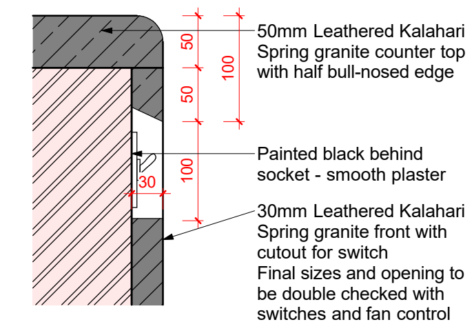
⑨ Callout - Switches cut out 1 : 5
