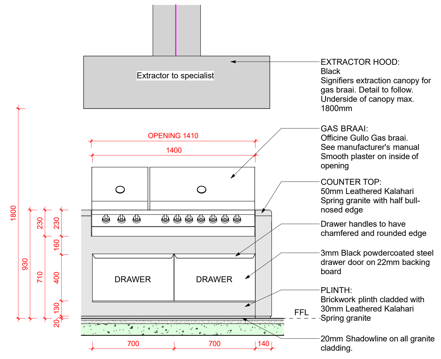
④ Elevation 04 - Gas Braai & Extractor 1 : 20
