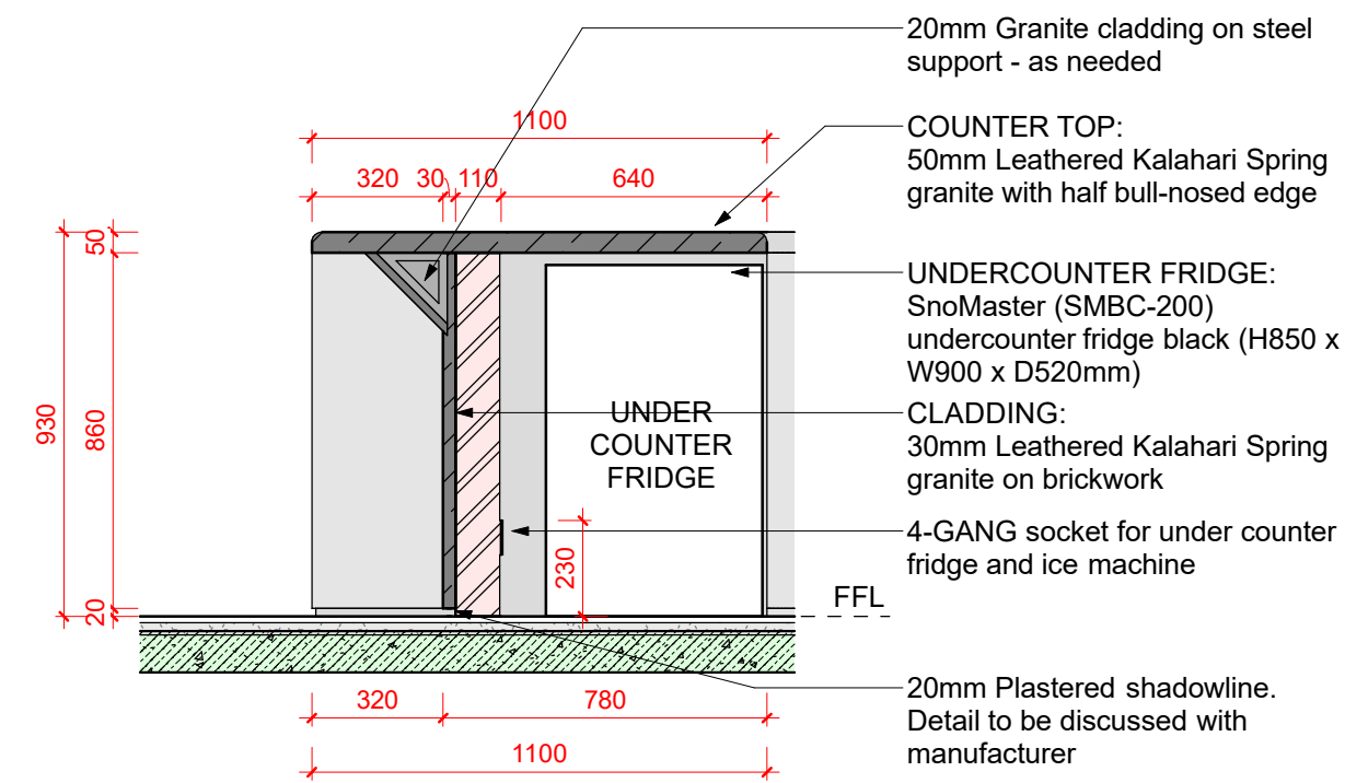
⑬ Section 06 - Bar Seating & Fridge 1 : 20
