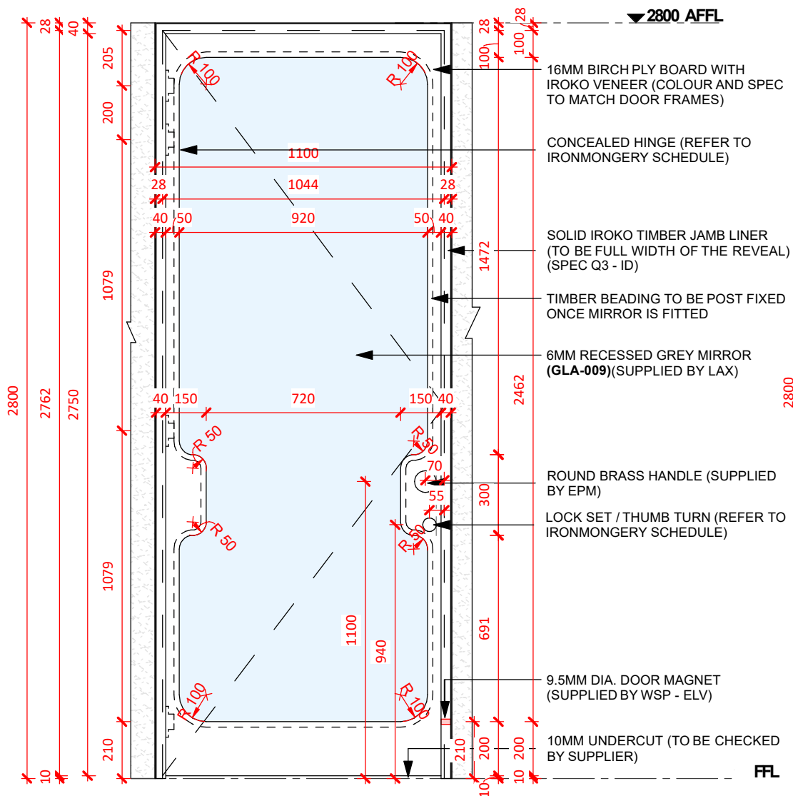
View A - Door Detail Elevation | 1:20
