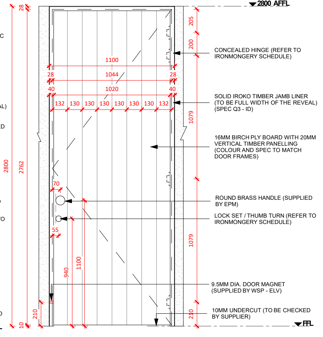
View B - Door Detail Elevation | 1:20
