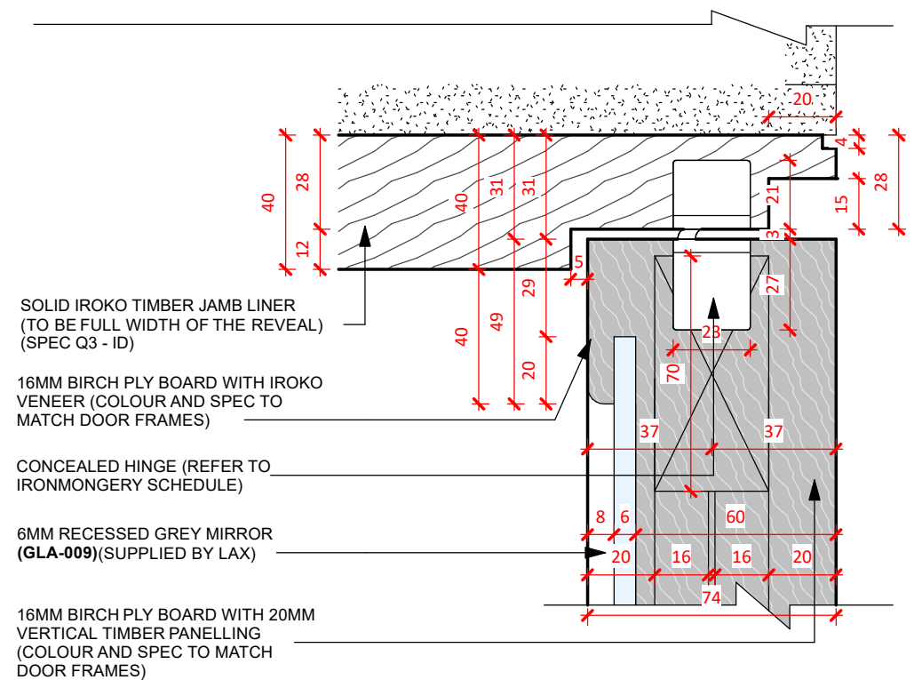
View B - Door Detail Elevation | 1:20
