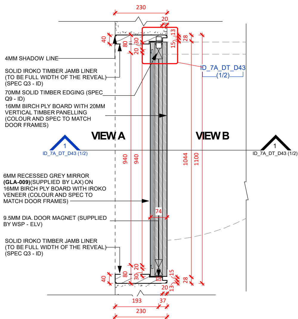
Plan - Single Hinge Door | 1:10
