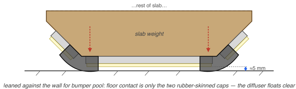
Leaned on its side — the caps carry the weight, not the LEDs
