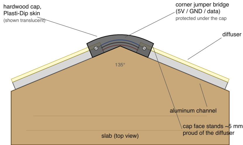
Top view — one of 8 corners
