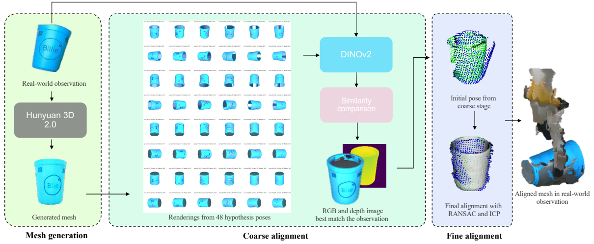
Fig. 2. The proposed digital twin construction module, containing the mesh generation and two-stage pose alignment. We first generate a textured mesh from the masked RGB image via Hunyuan3D 2.0 [24]. During coarse alignment, we render RGB and depth images from a set of hypothesis poses and compare their similarities with real-world observation in DINO [25] feature space, and select the one that best matches the real-world observation. The resulting coarse pose is then refined using RANSAC and ICP on the partial point cloud back-projected from the depth image.
