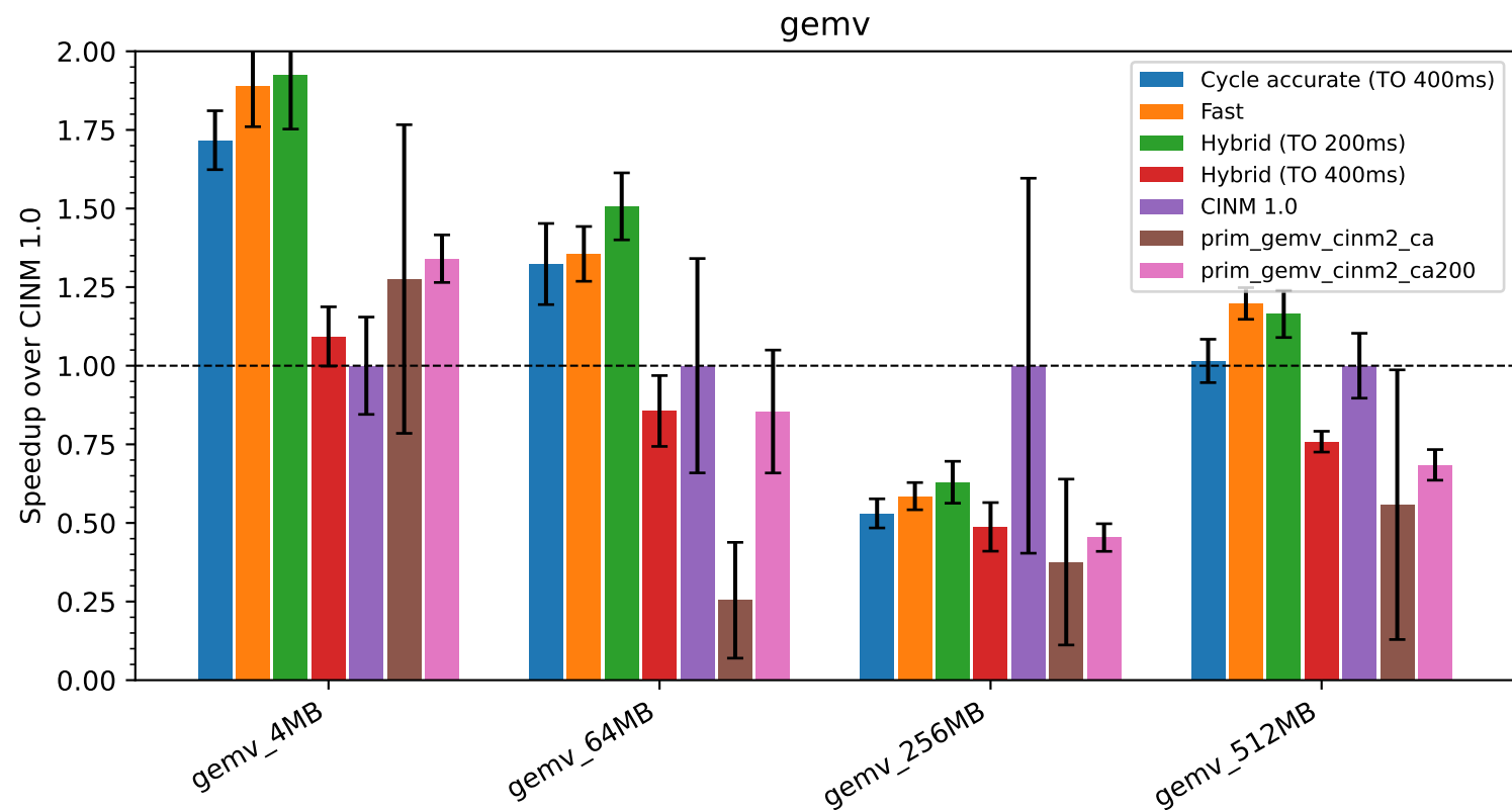
Speedup over CINM 1.0 (BO-search timings, mean \pm std over seeds)
