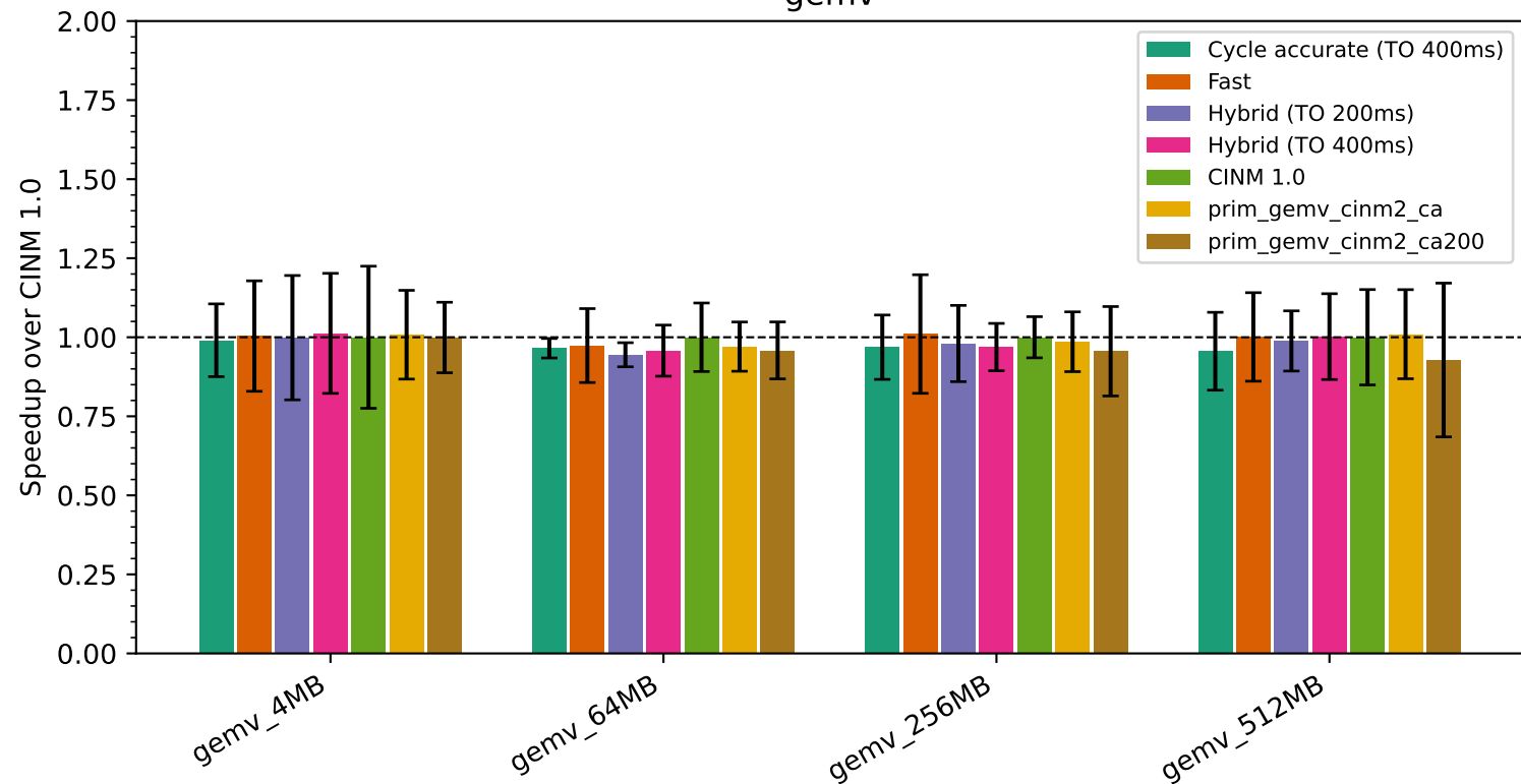
Speedup over CINM 1.0 (net execution time, mean \pm std over seeds)
