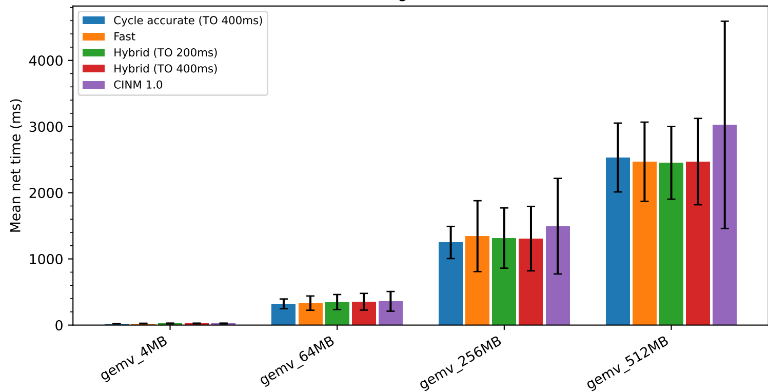
Mean net execution time \pm std over seeds
