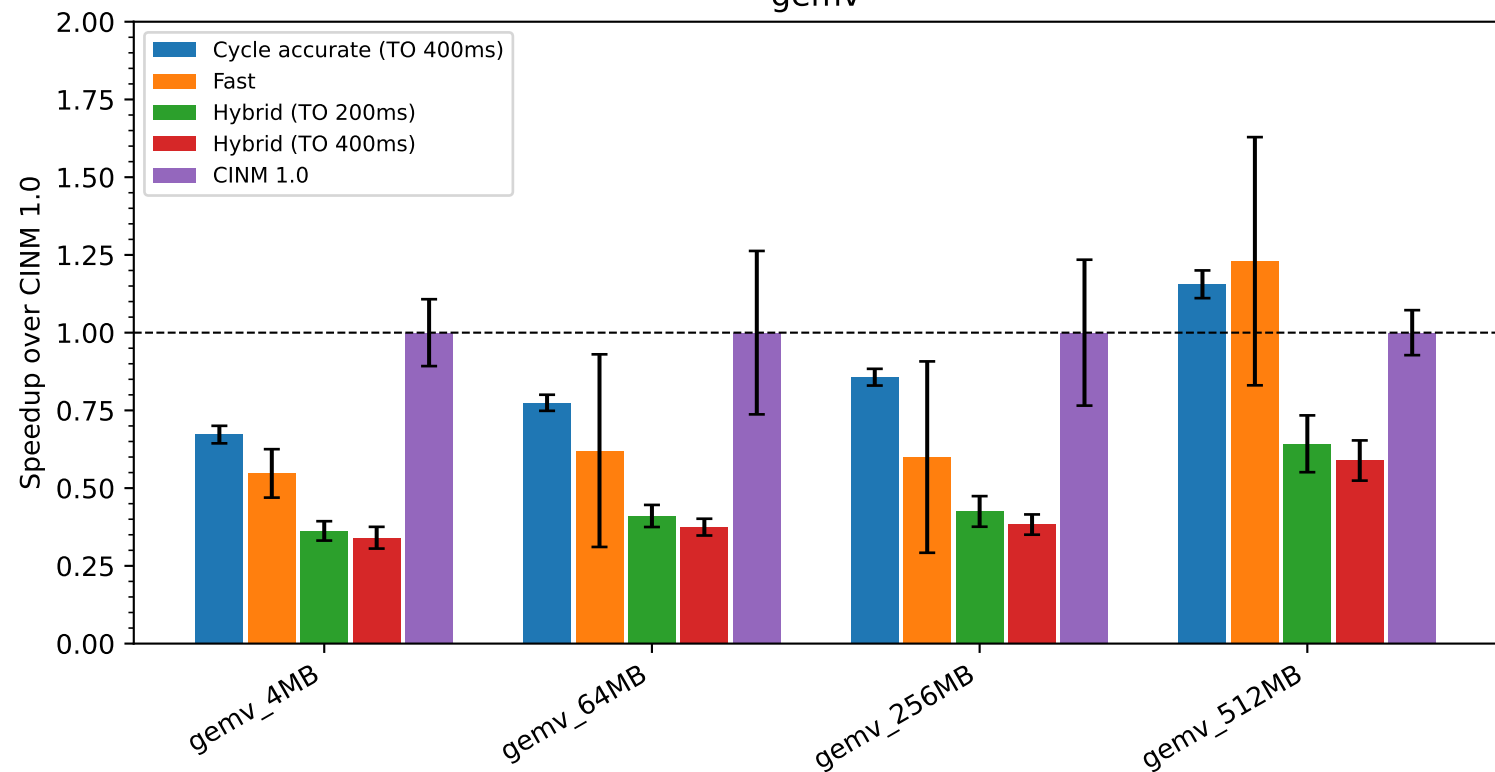
Speedup over CINM 1.0 (BO-search timings, mean \pm std over seeds)
