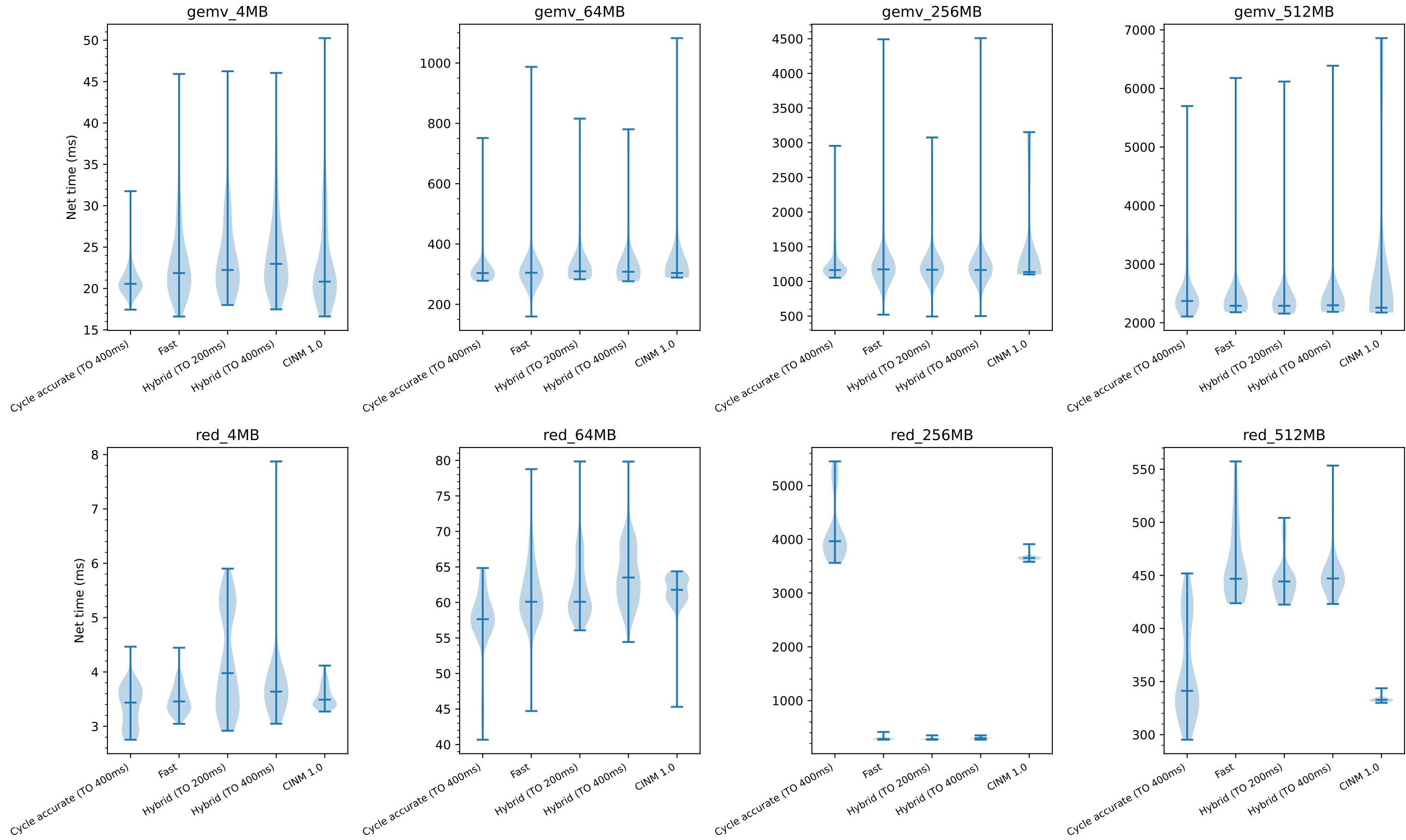
Net execution time per source and problem size
