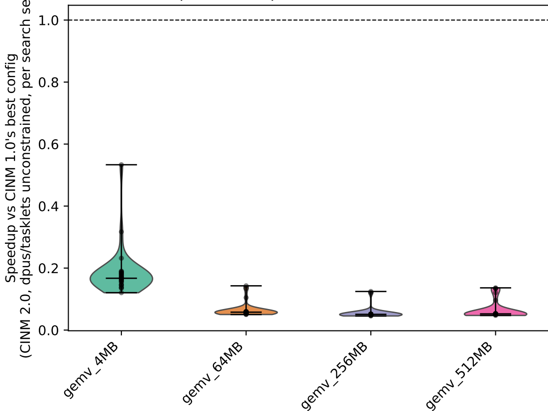
CINM 2.0 (free search) vs CINM 1.0's best-ever config, per benchmark (spread: independent search seeds)
