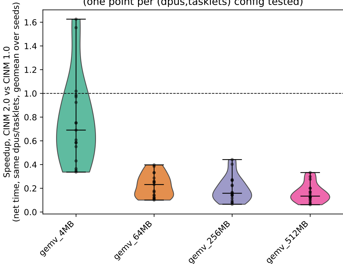
CINM 2.0 vs CINM 1.0 codegen at matched hardware configs (one point per (dpus,tasklets) config tested)
