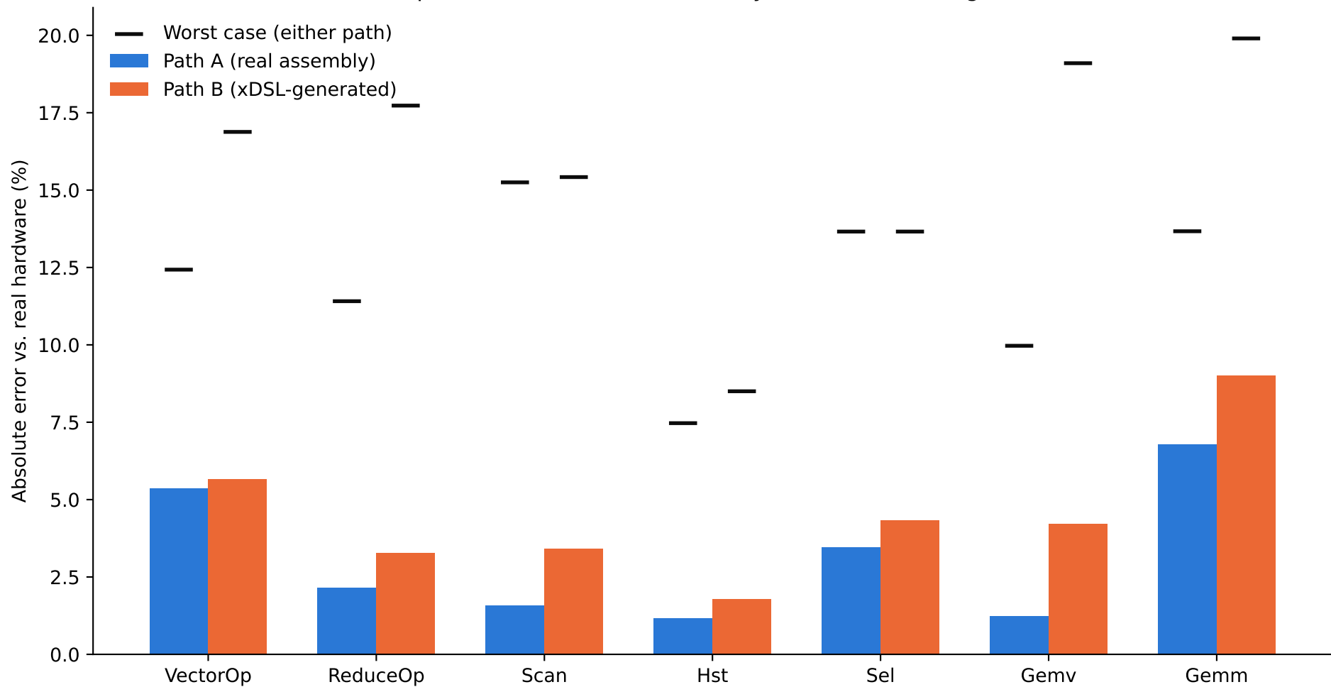
Cost-model prediction error: real-assembly-derived vs xDSL-generated code
