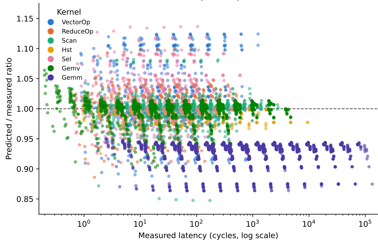
Prediction ratio vs. measured latency, all kernels (dashed line = perfect prediction)
