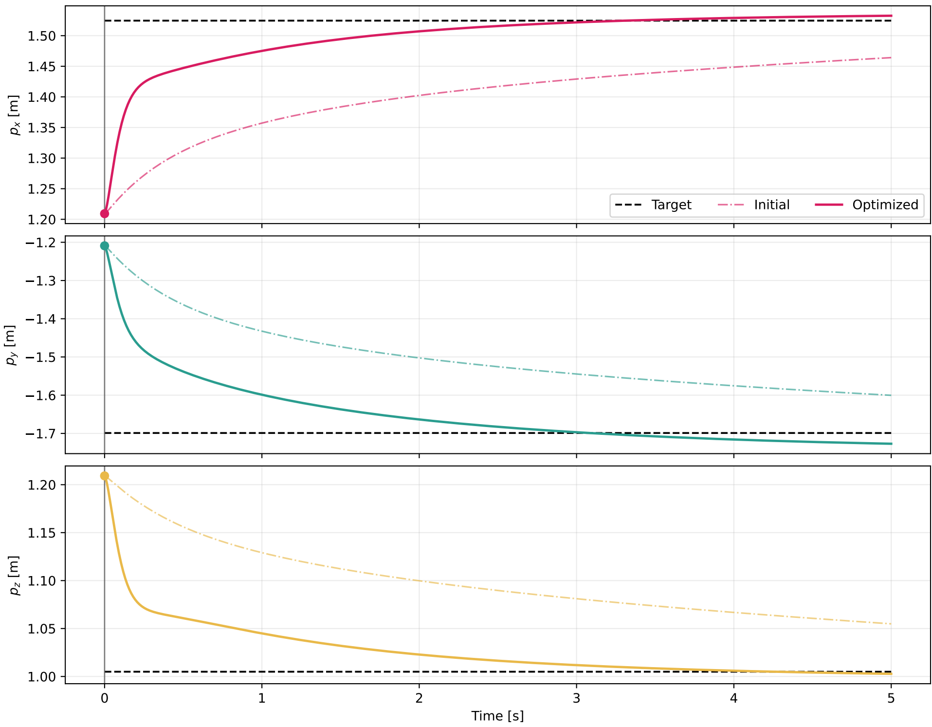
Synergistic end-effector tracking — best batch 1
