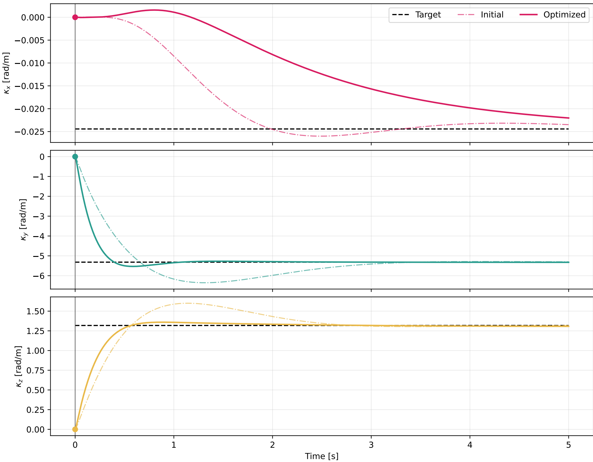
Collocated strain tracking — best batch 4
