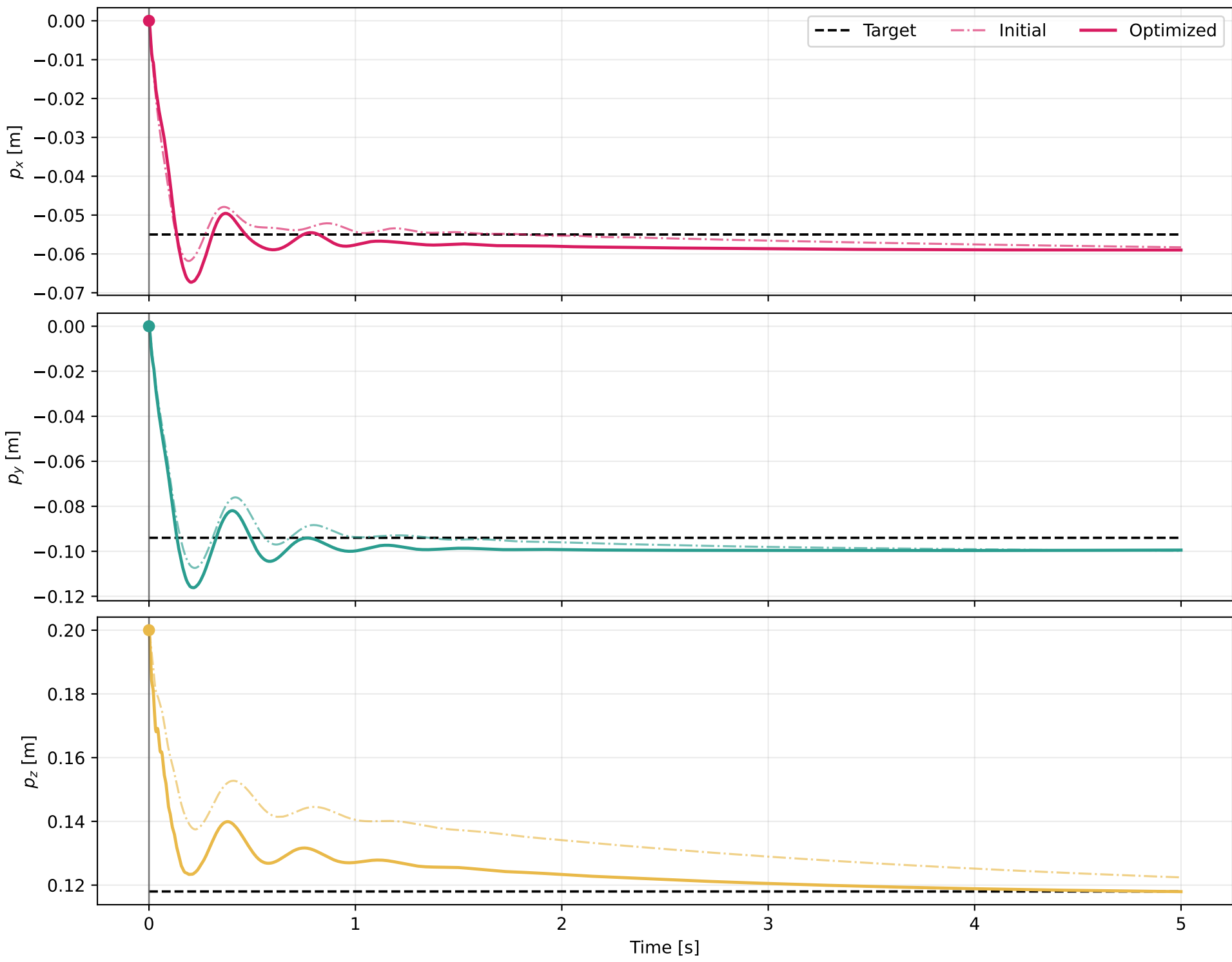
Synergistic end-effector tracking — best batch 4
