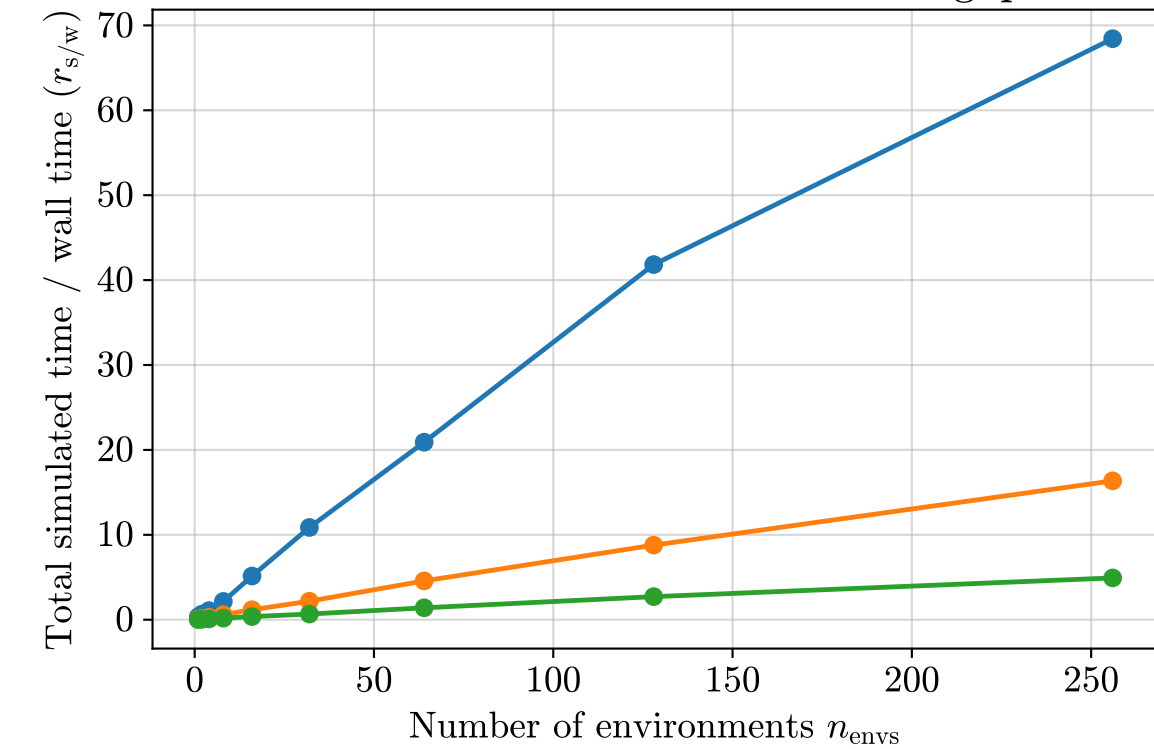
Articulated Soft Robot - total throughput
