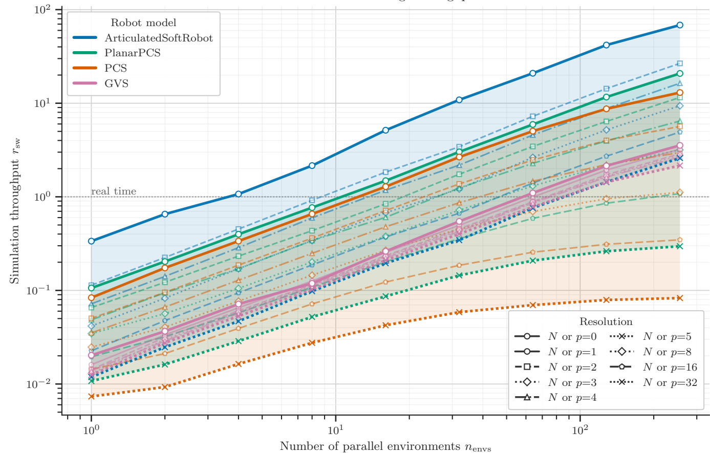
GPU Batch-Scaling Throughput
