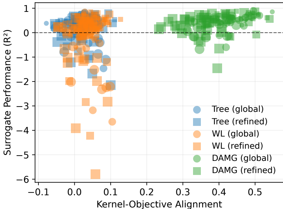
Kernel Alignment and Surrogate Performance
