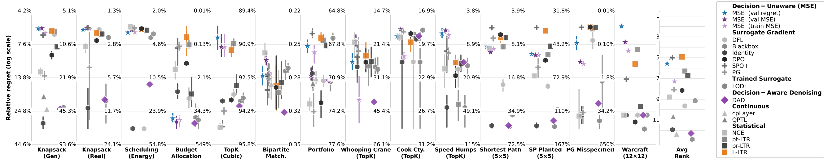
Benchmark re-run — All 14 tasks — mean \pm 95% bootstrap CI of mean (n \leq 10 seeds) — Relative regret % (best \uparrow )
