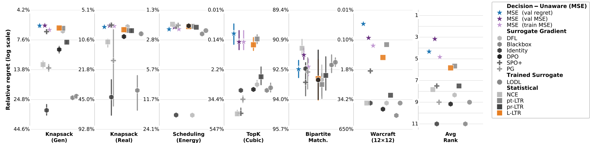
Benchmark re-run — 10-seed mean \pm 95% bootstrap CI — Relative regret % (best \uparrow )
