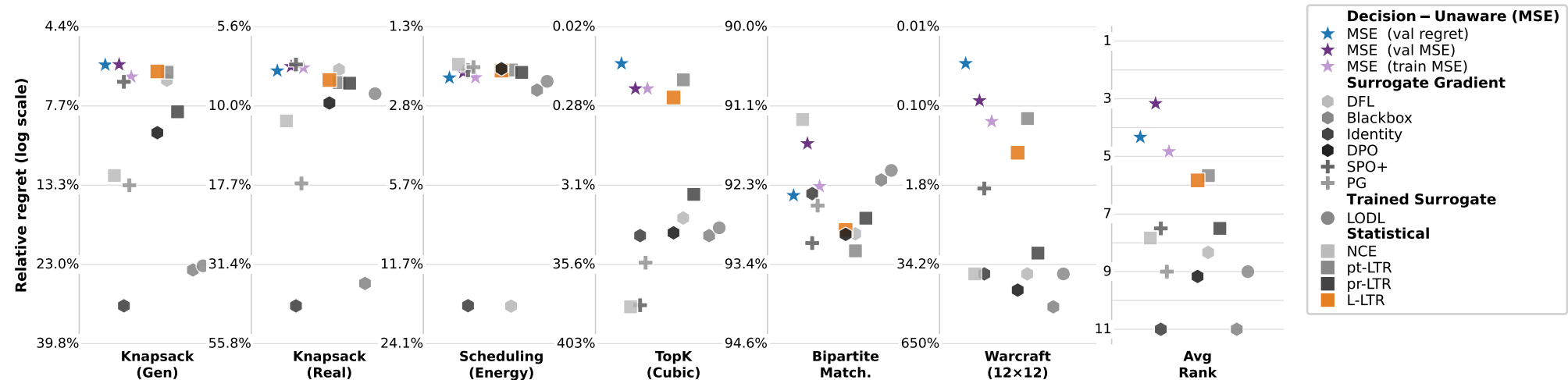
Benchmark re-run — 10-seed mean — Relative regret % (best ↑)
