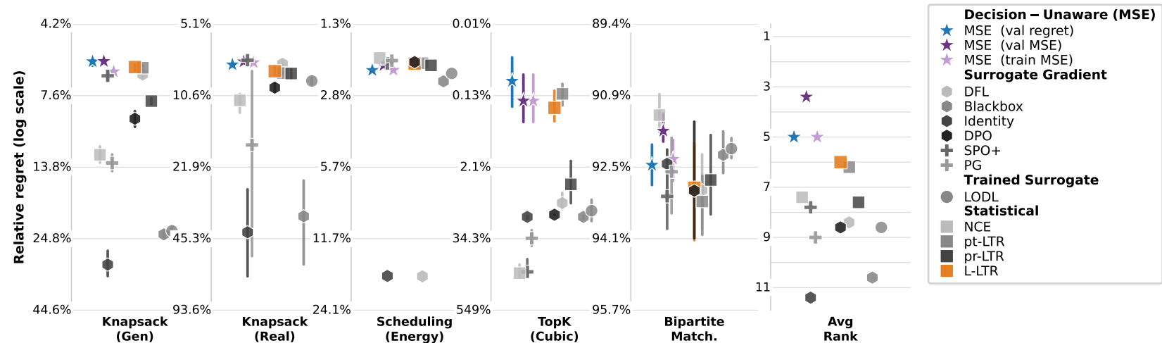
Benchmark re-run — Classic tasks — mean \pm 95% bootstrap CI of mean — Relative regret % (best \uparrow )
