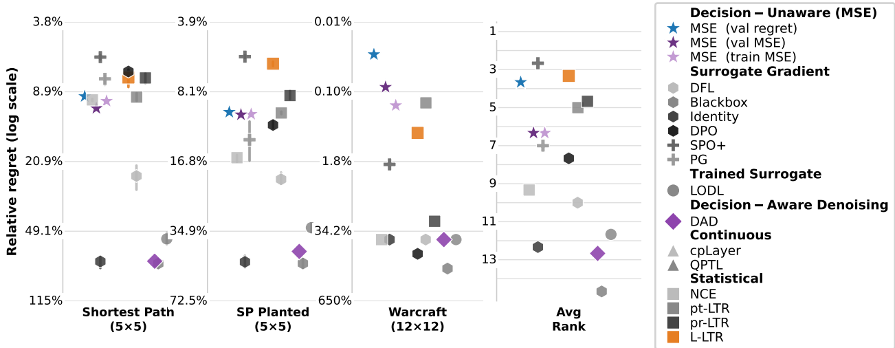
Benchmark re-run — Shortest-path tasks — mean \pm 95% bootstrap CI of mean
