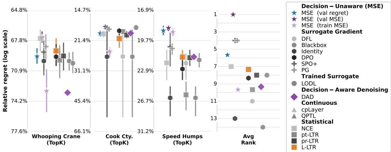
Benchmark re-run — Spatial TopK tasks — mean \pm 95% bootstrap CI of mean
