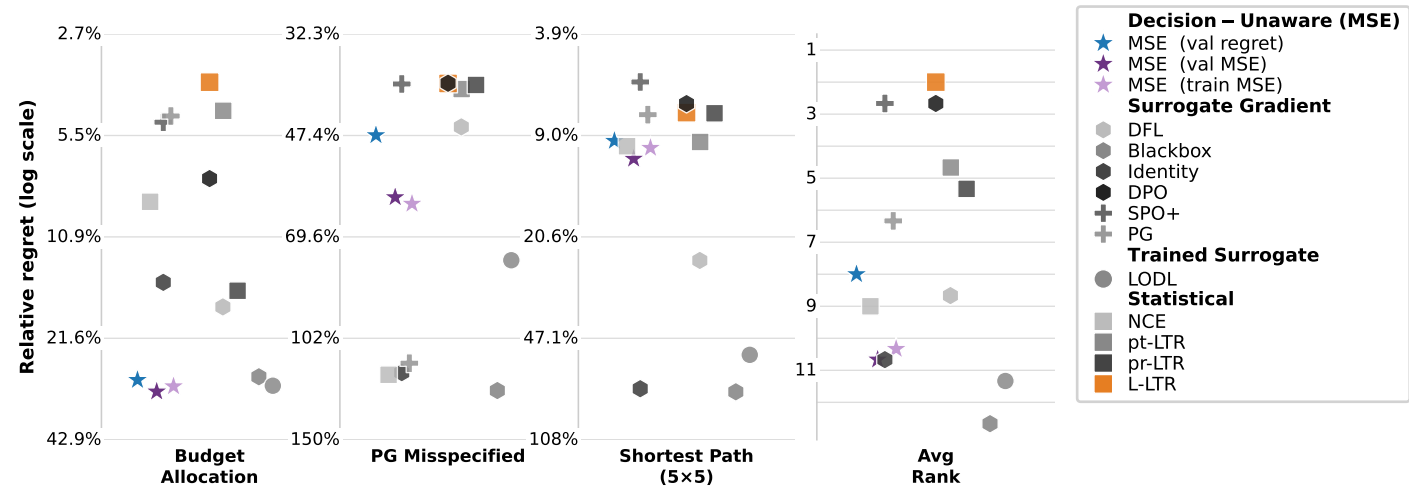
Benchmark re-run — 10-seed mean — Relative regret % (best ↑)
