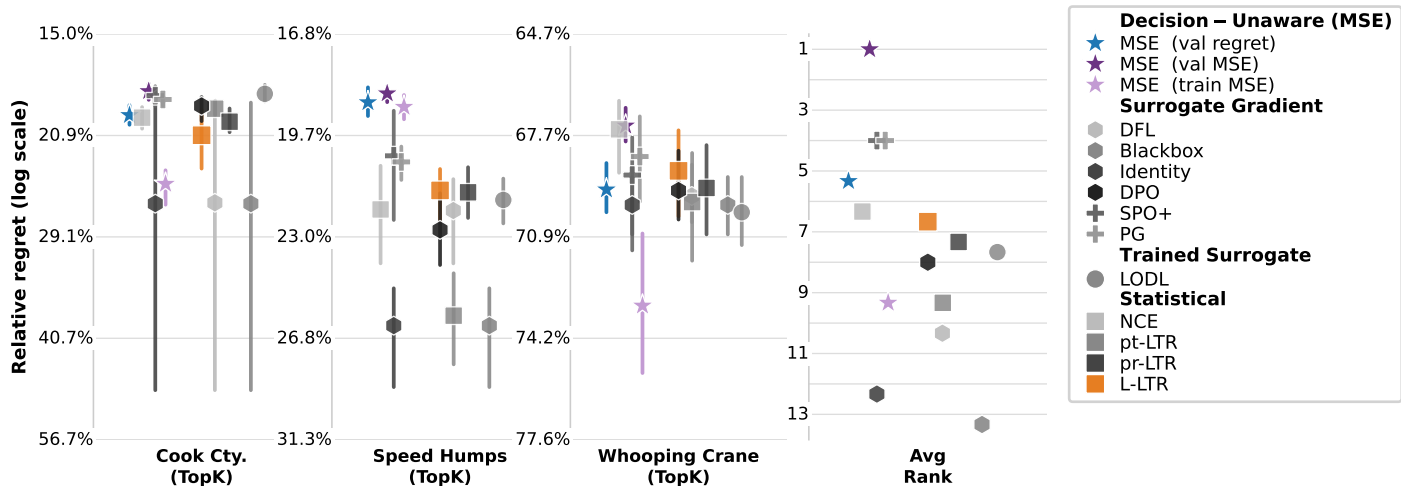
Benchmark re-run — 10-seed mean \pm 95% bootstrap CI — Relative regret % (best \uparrow )
