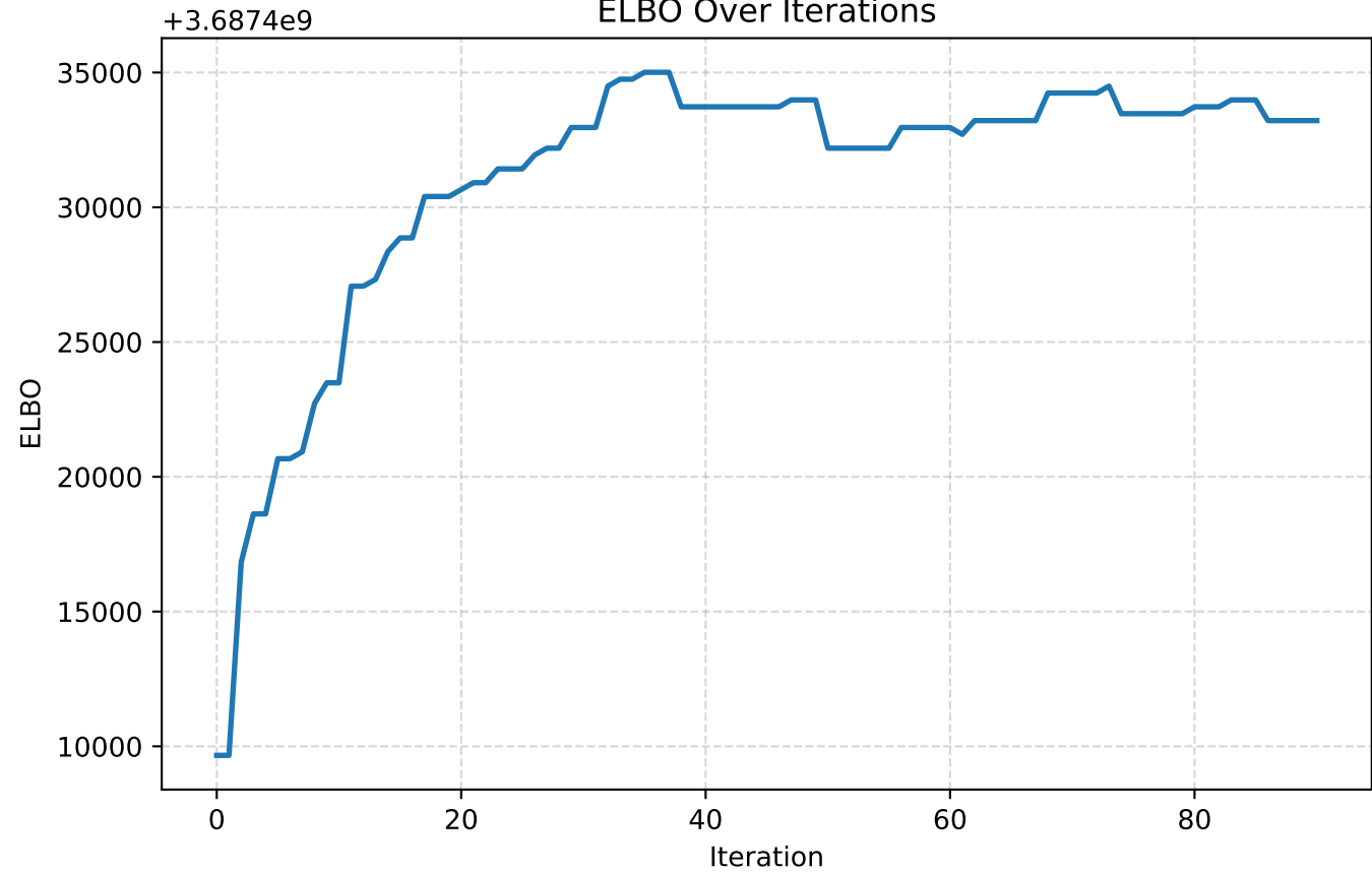
ELBO Over Iterations
