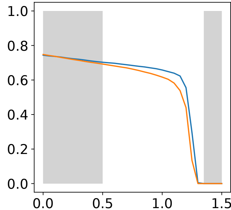
CIFAR-100
