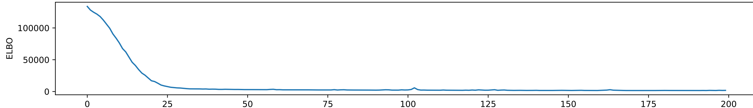
ELBO LOSS
