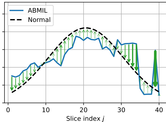
Reverse KL (mode-covering)
