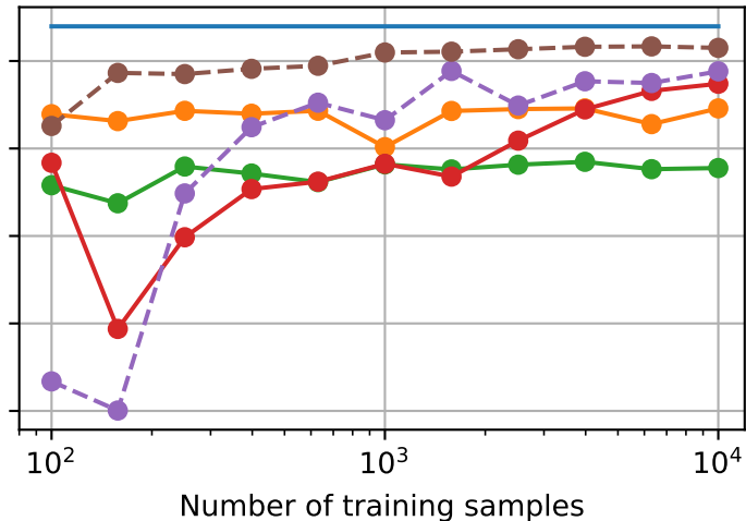
Embedding-aggregation approach
