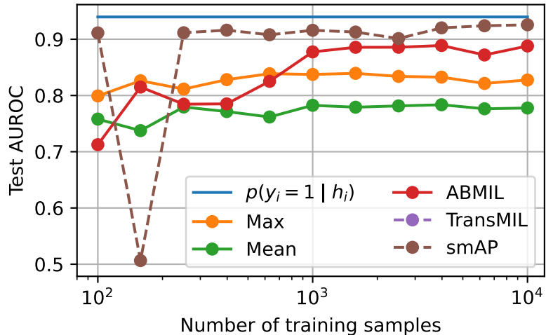
Prediction-aggregation approach
