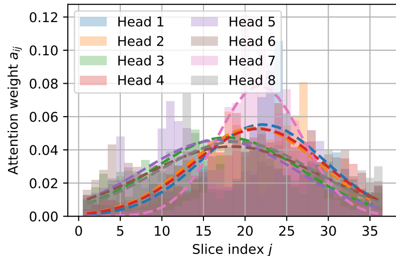
Multi-Head Normal Guidance
