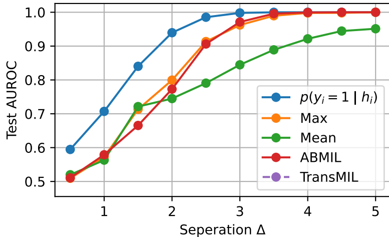
Prediction-aggregation approach
