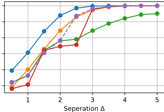
Embedding-aggregation approach
