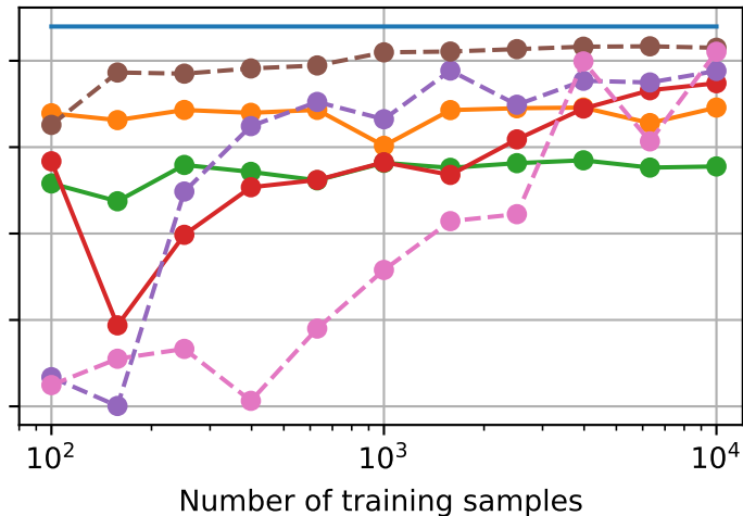
Embedding-aggregation approach
