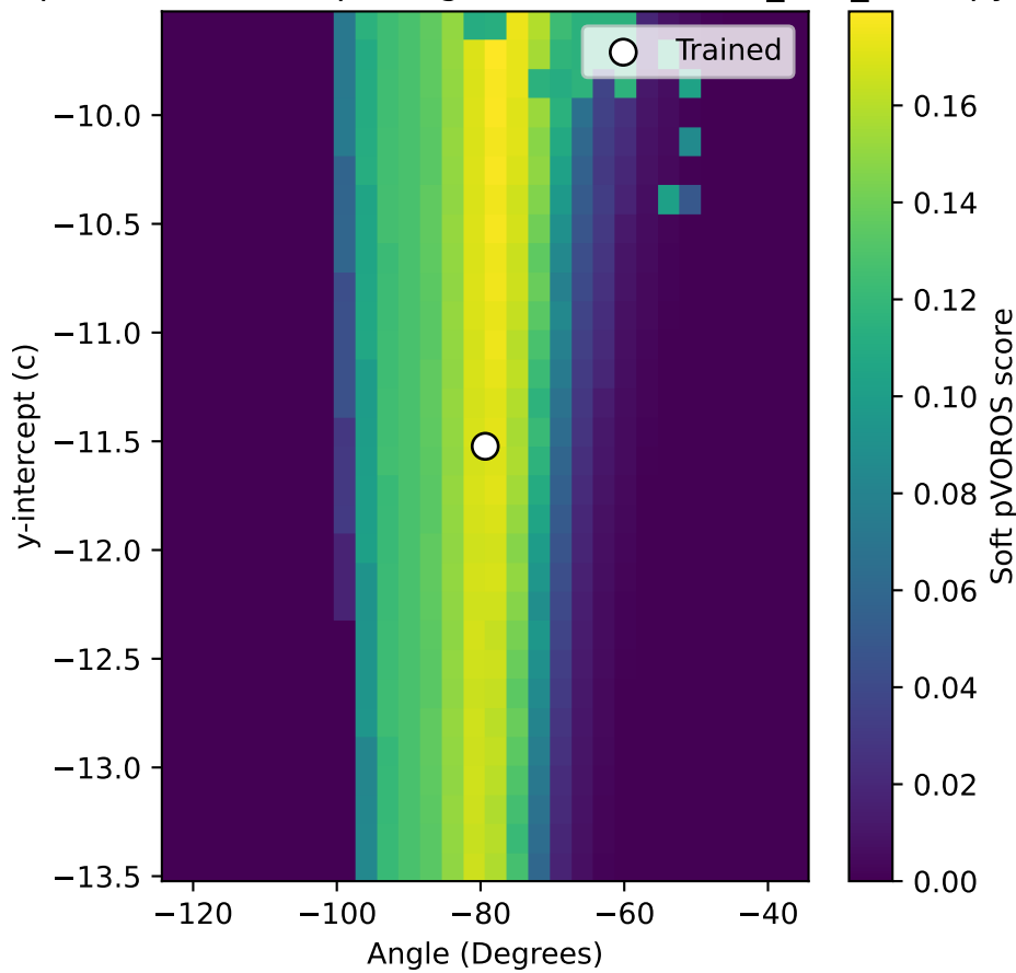
Soft pVOROS Heatmap (magnitude = 1): seed_601_201.npy
