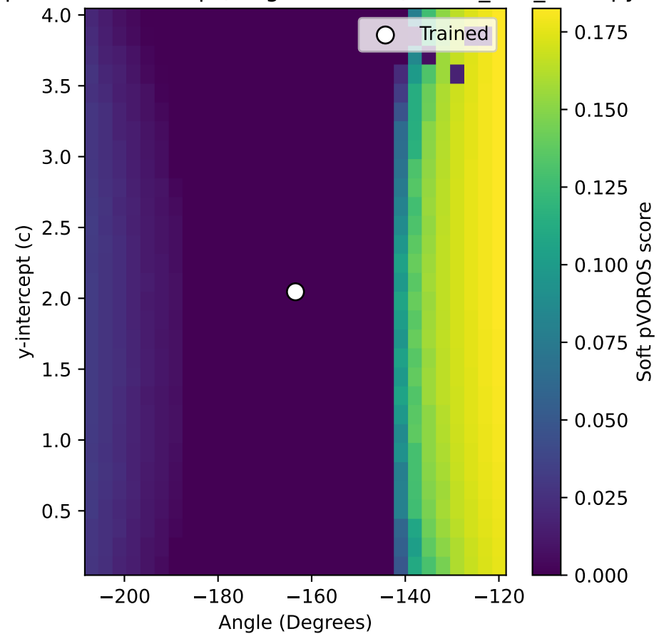
Soft pVOROS Heatmap (magnitude = 1): seed_501_801.npy
