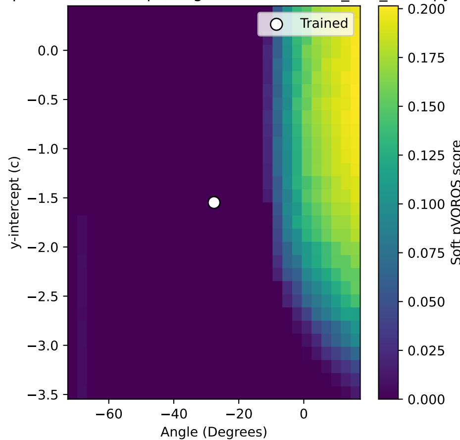
Soft pVOROS Heatmap (magnitude = 1): seed_701_501.npy
