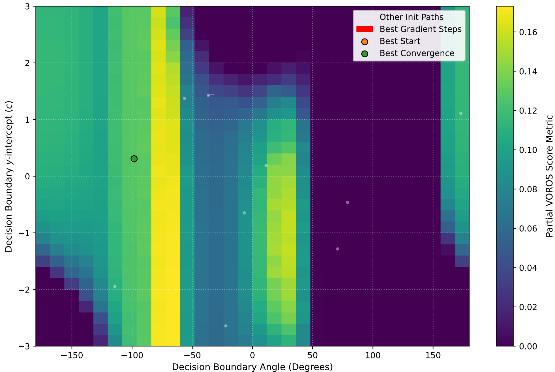
Gradient Descent Path: seed_601_201.npy (Best: Trial 2) Held Constant Vector Norm ||w|| = 1.0
