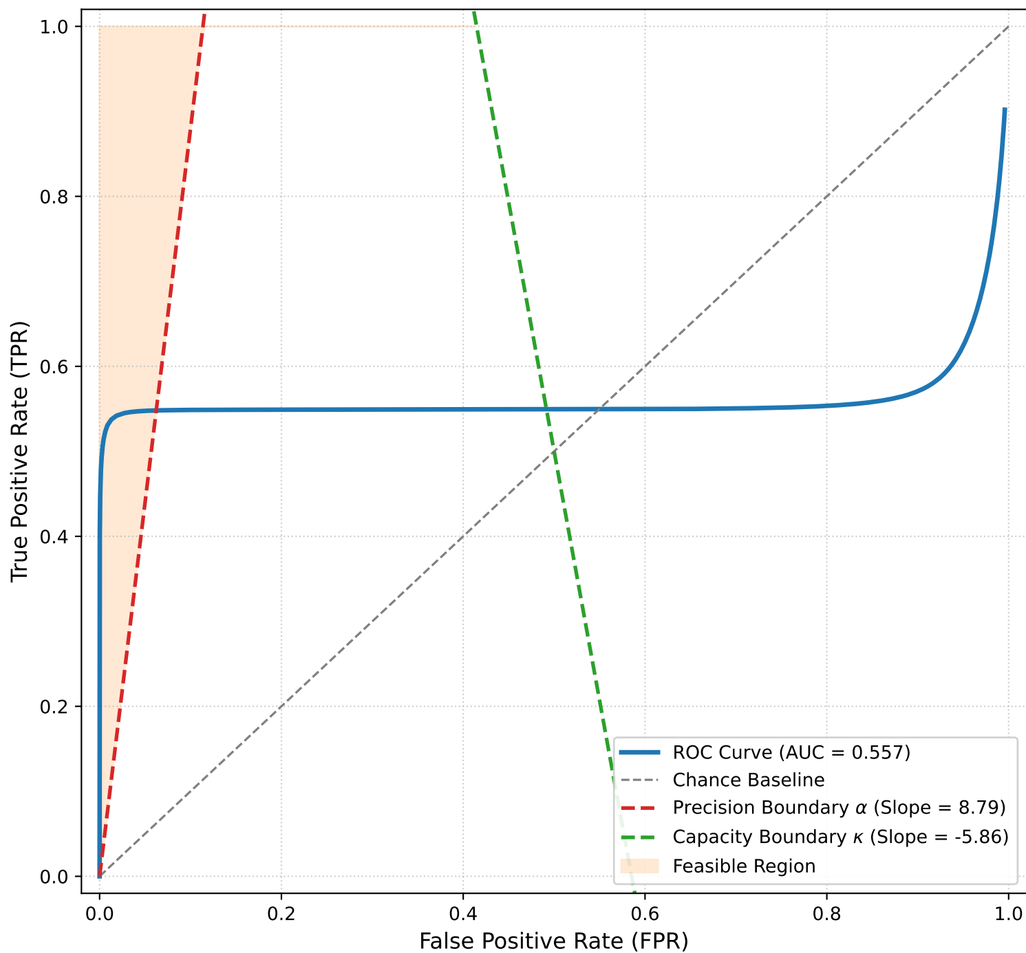
ROC Curve with Dual Slope Bounds ( \alpha & \kappa ): seed_101_201.npy Optimal \theta : 57.2°, c : -1.294
