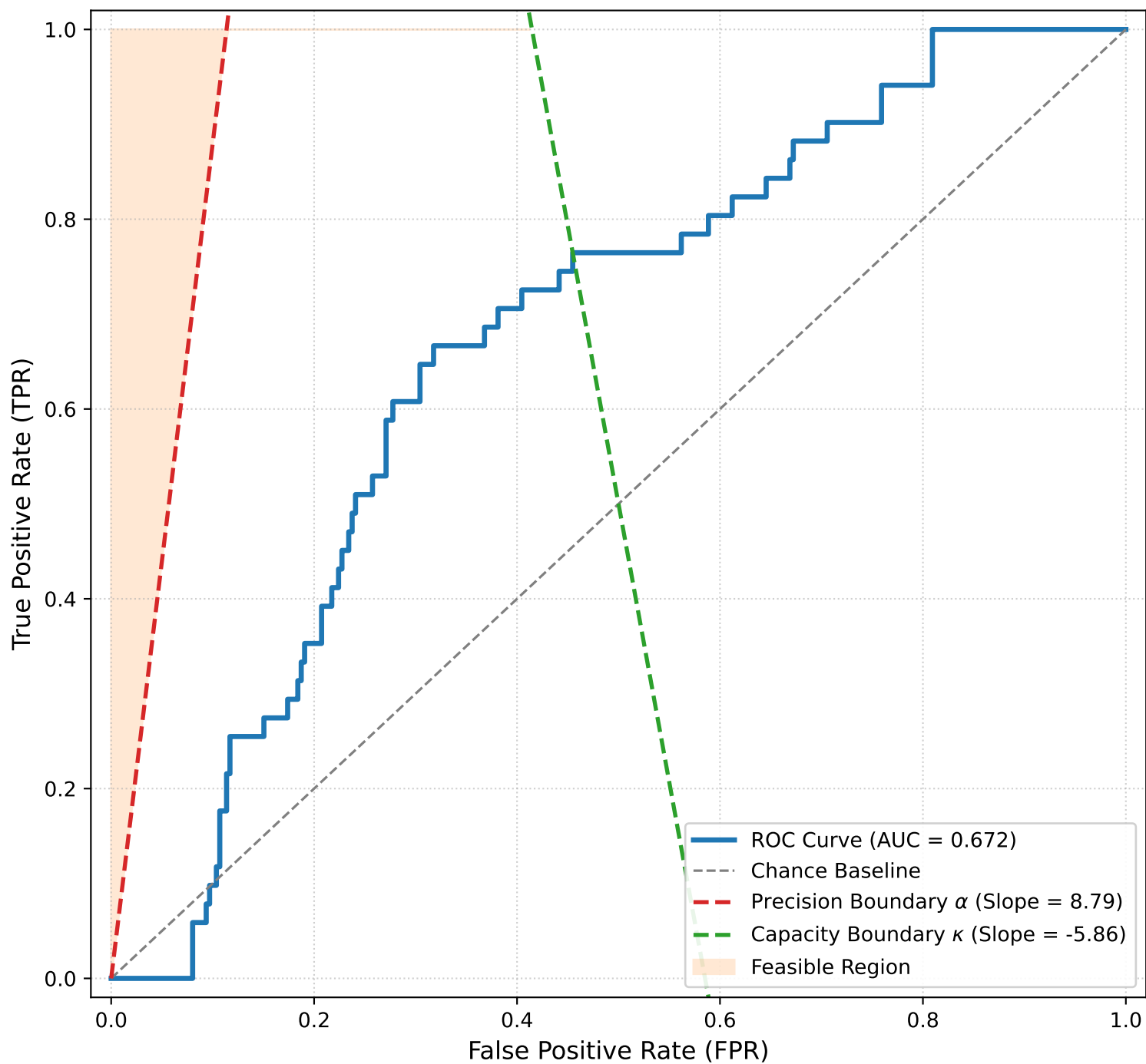
ROC Curve with Dual Slope Bounds ( \alpha & \kappa ): seed_701_501.npy Optimal \theta : 70.7°, c : -1.283
