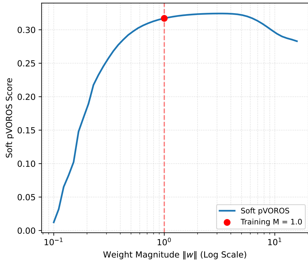
Seed: seed_101_201 ( \theta^* = 57.2^\circ, c^* = -1.29 )
