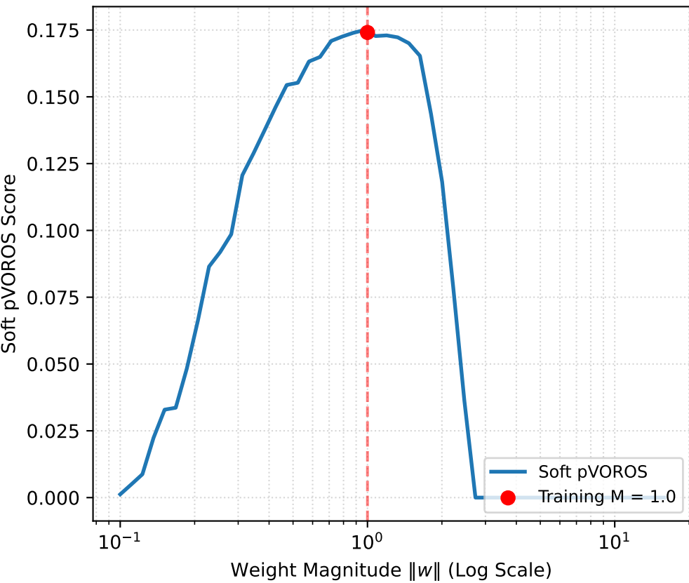
Seed: seed_601_201 ( \theta^* = -73.6^\circ, c^* = 1.43 )
