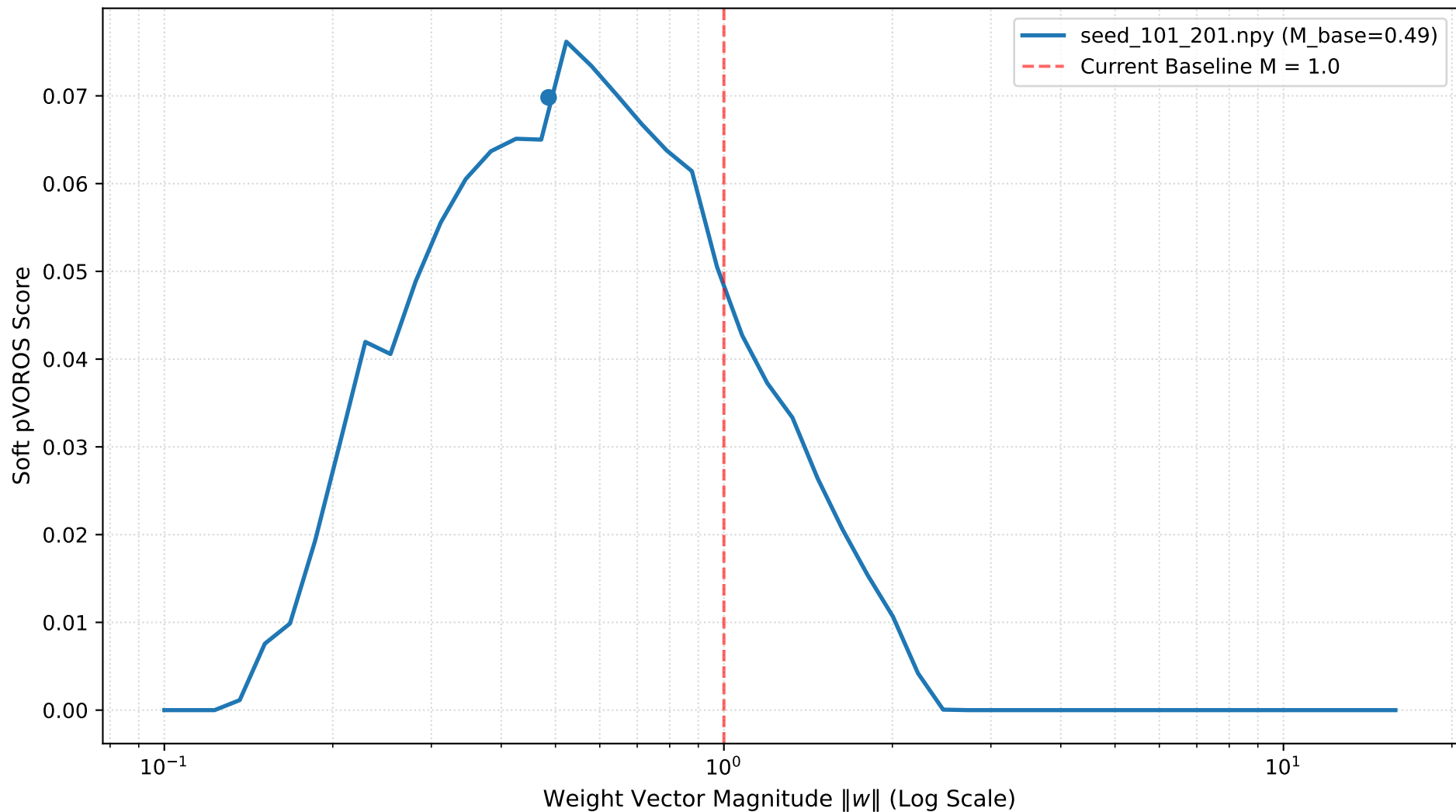
Soft pVOROS Score vs. Weight Magnitude \|w\|
