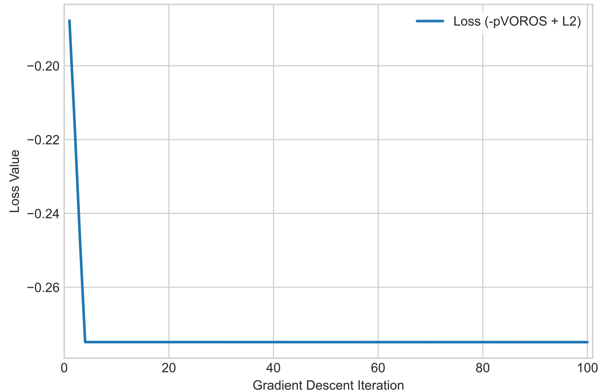
Training Loss
