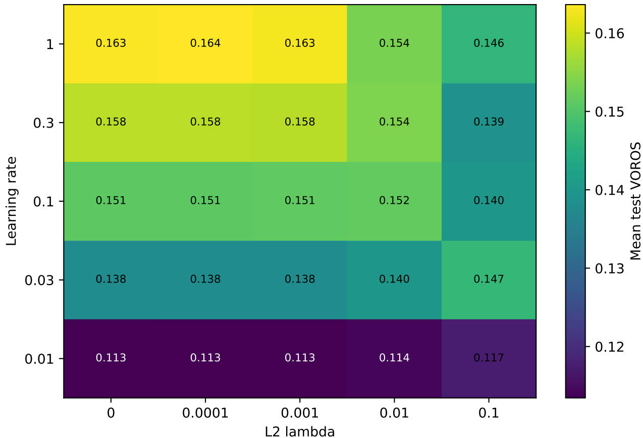
Mean held-out VOROS by (learning rate, L2 lambda)
