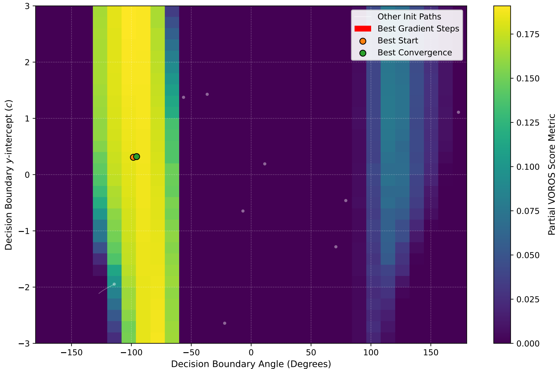
Gradient Descent Path: seed_501_801.npy (Best: Trial 2) Held Constant Vector Norm ||w|| = 1.0
