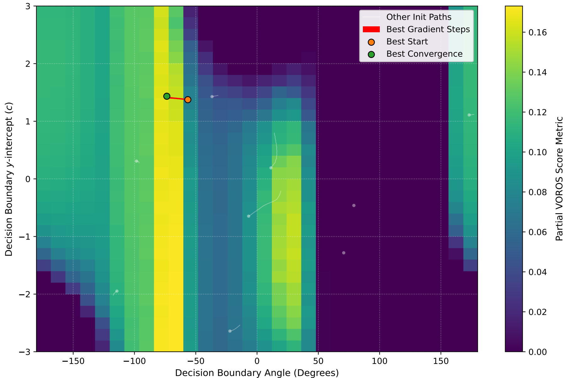
Gradient Descent Path: seed_601_201.npy (Best: Trial 6) Held Constant Vector Norm ||w|| = 1.0
