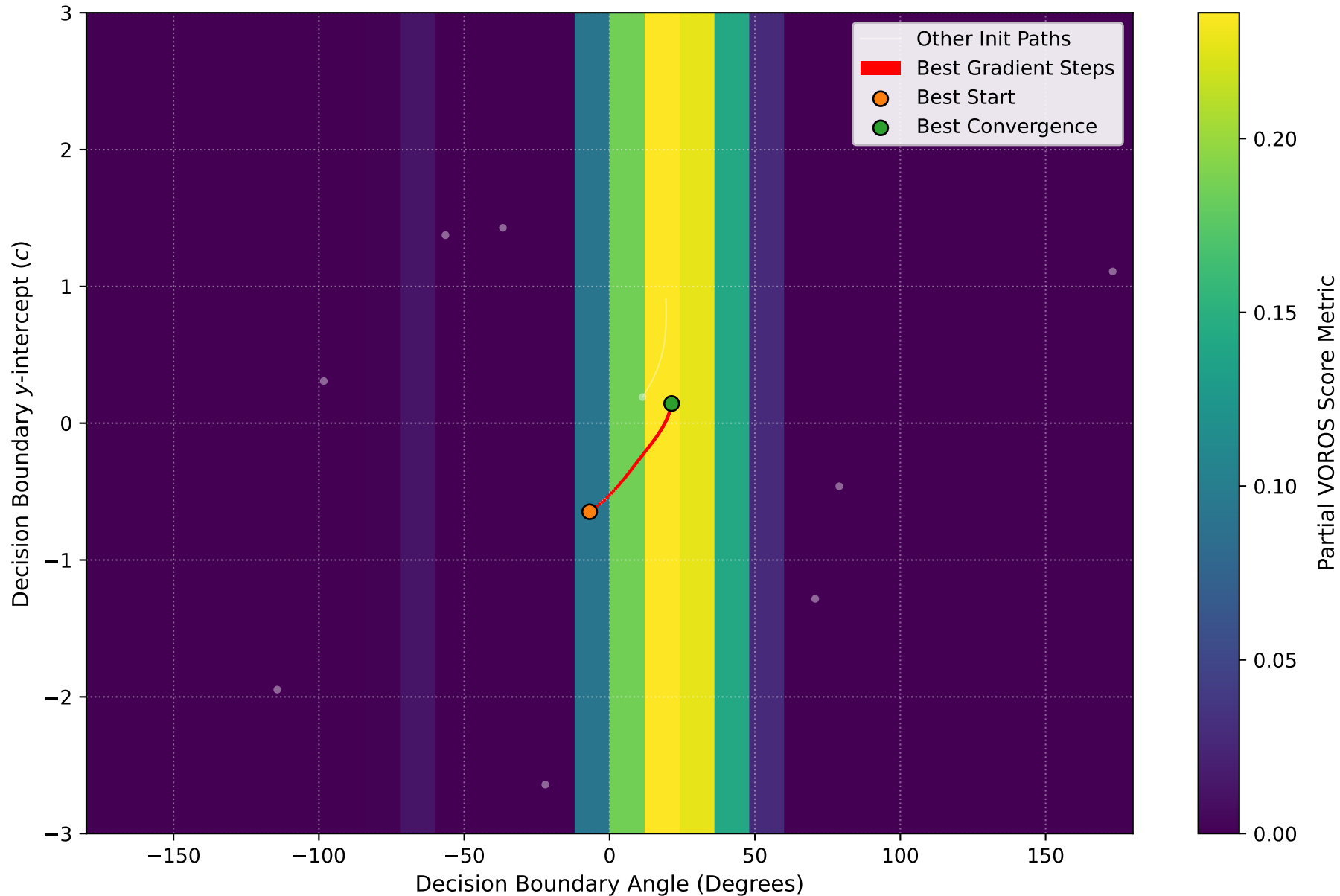
Gradient Descent Path: seed_301_101.npy (Best: Trial 5) Held Constant Vector Norm ||w|| = 1.0
