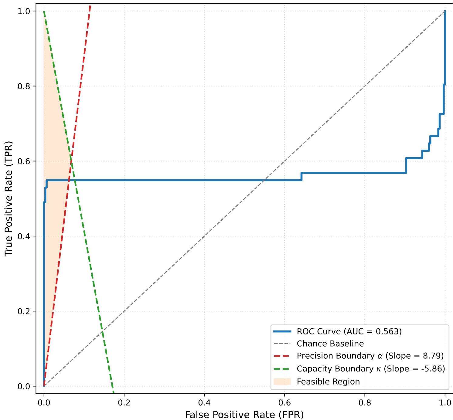
ROC Curve with Dual Slope Bounds ( \alpha & \kappa ): seed_101_201.npy Optimal \theta : 70.7°, c : -1.283
